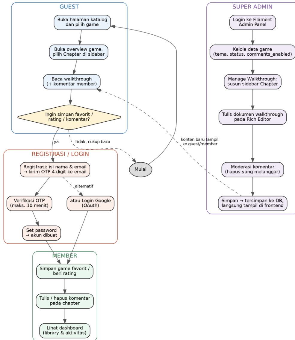
Gambar: Flowchart alur proses bisnis Guest, Registrasi/Login, Member, dan Super Admin.
