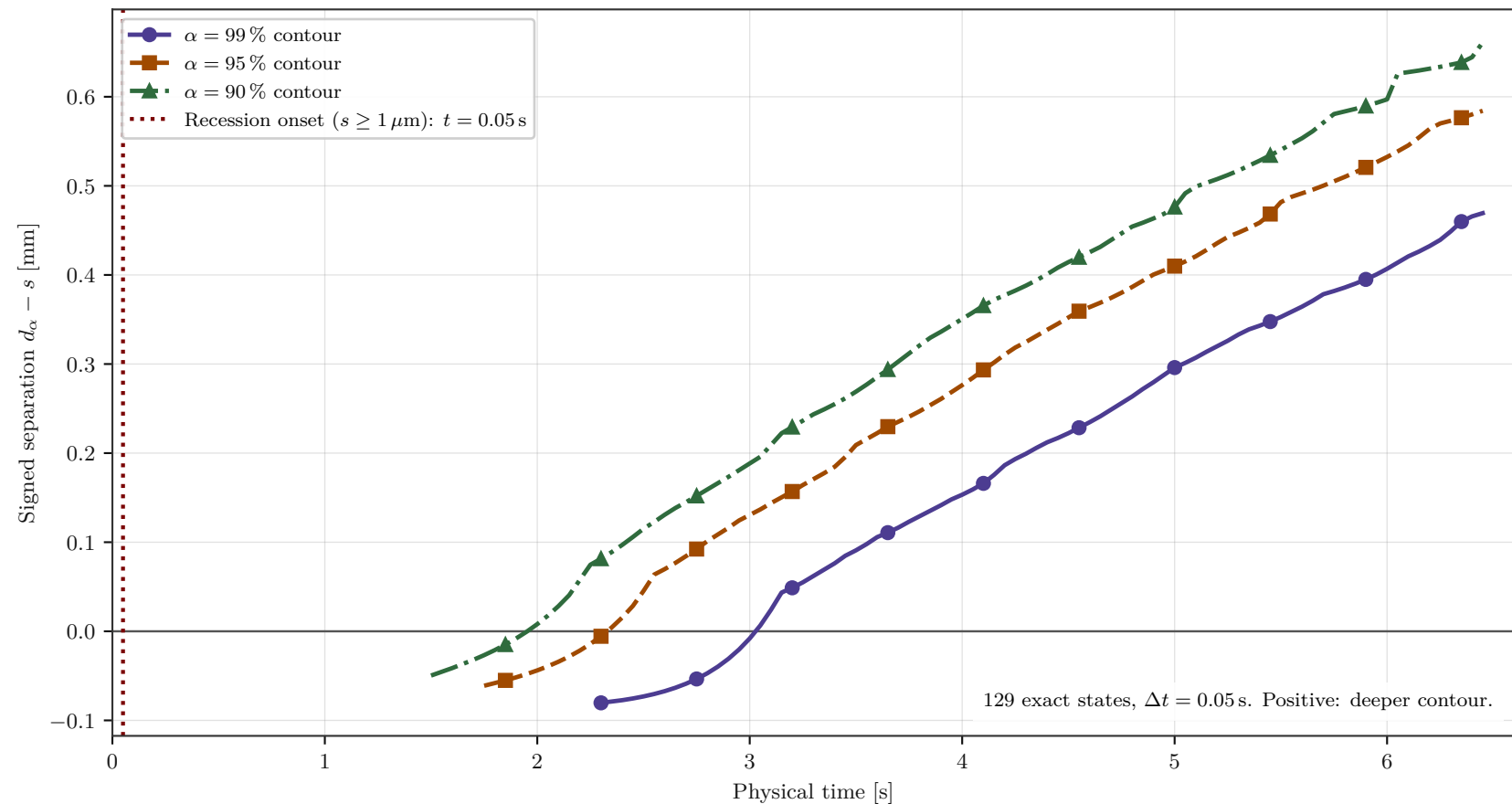
Simulation 2: radial separation between virtual recession and pyrolysis-conversion contours
