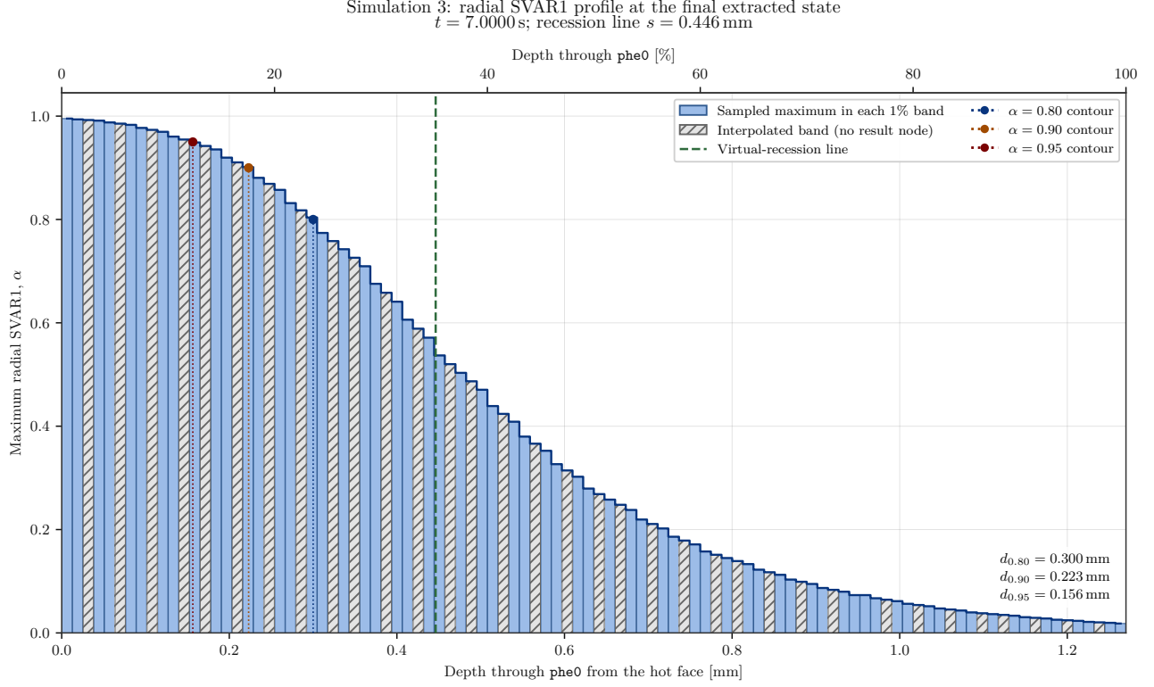
Figure 25. Final radial SVAR1 profile at 7 s, including conversion contours and the virtual-recession line.
