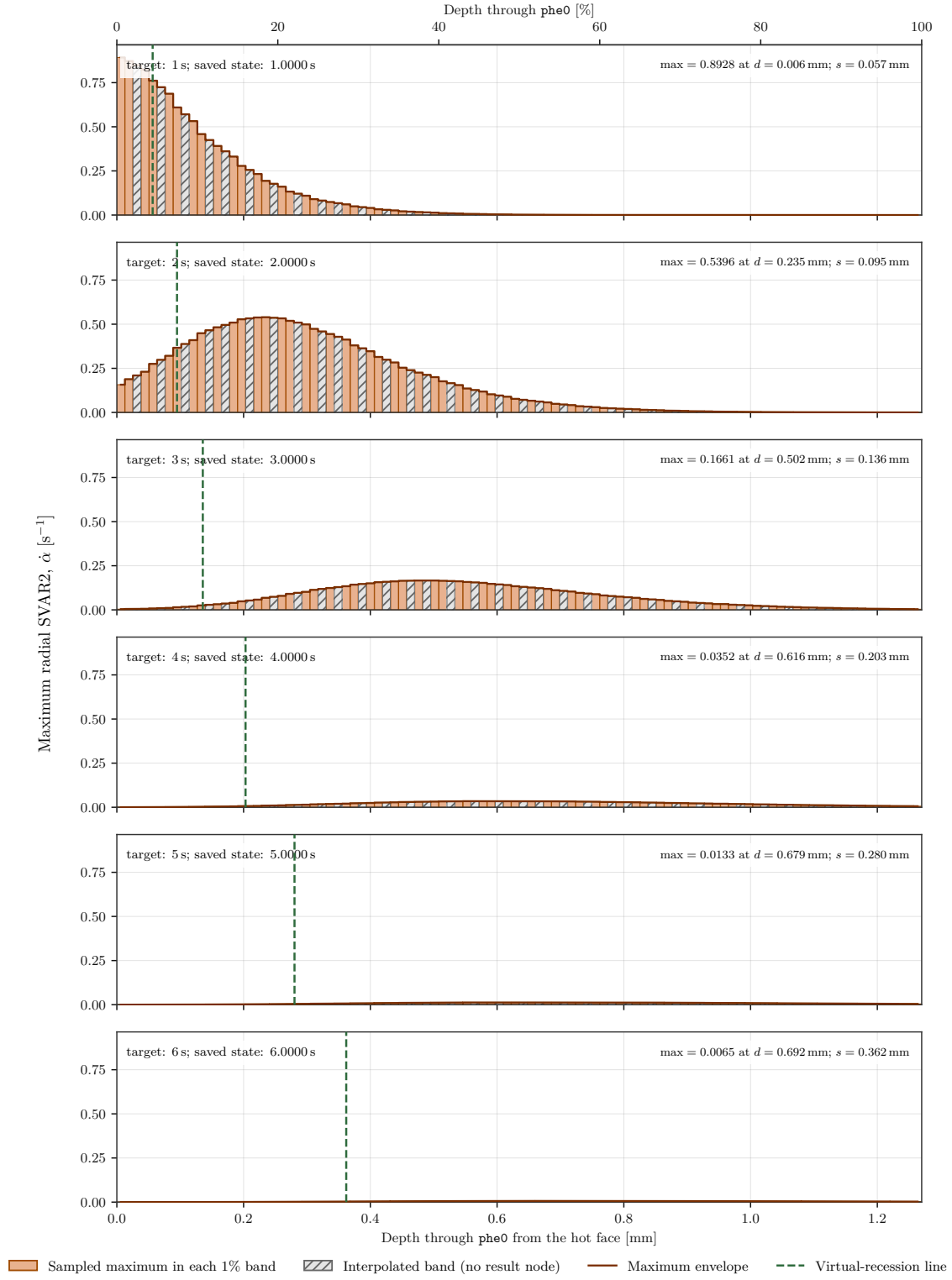
Figure 27. Evolution of radial SVAR2 profiles; the maximum identifies the region where pyrolysis remains active.
