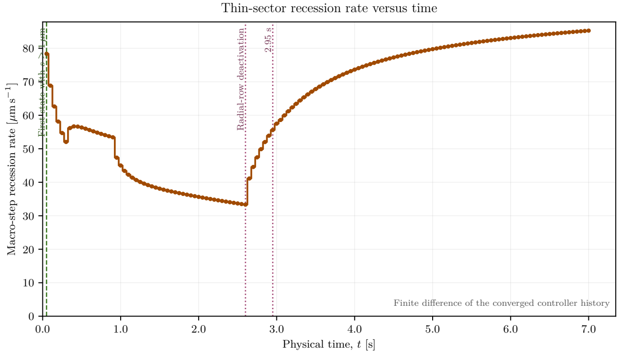
Figure 22. Macro-step recession rate. This is a temporal derivative of the controller history, without a spatial standard-deviation bar.
