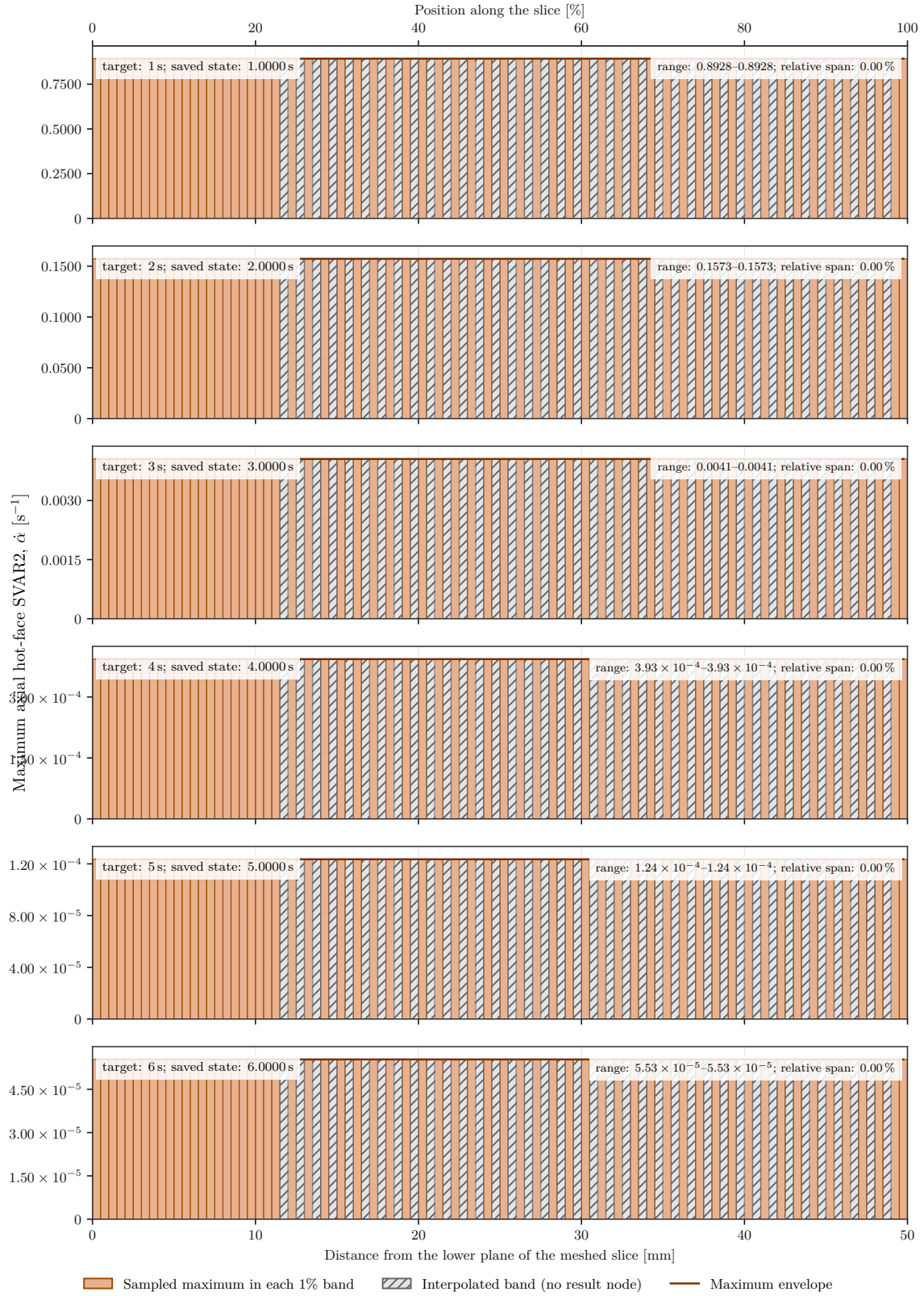
Figure 29. Axial uniformity of SVAR2 along the thin sector's hot face.
