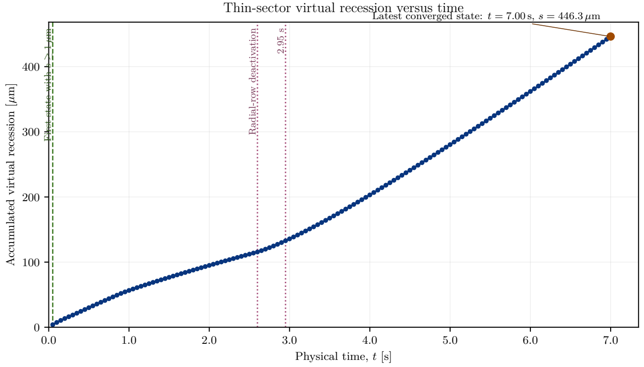
Figure 21. Accumulated virtual recession versus time for Simulation 3. The vertical lines mark numerical onset of the recession front and both radial-row deactivations.
