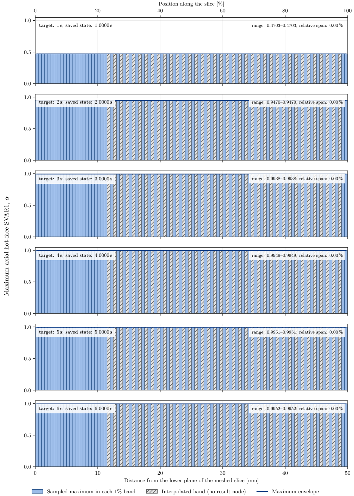
Figure 28. Axial uniformity of SVAR1 along the thin sector's hot face.
