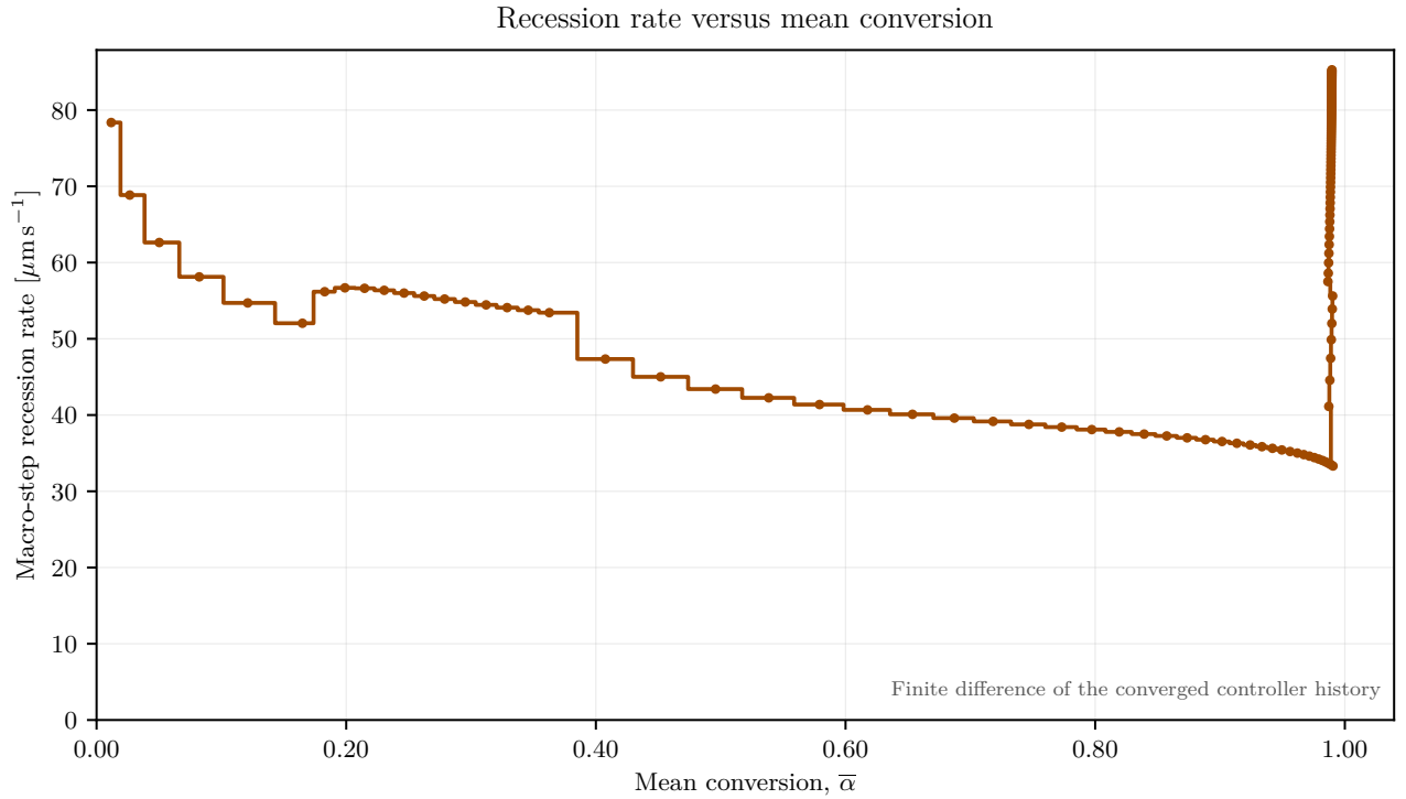
Figure 24. Macro-step recession rate versus mean conversion.
