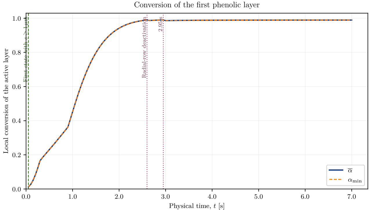
Figure 19. Mean and minimum conversion recorded in the thin sector’s active layer over all 140 converged states. Vertical lines mark the two radial-row deactivations.
