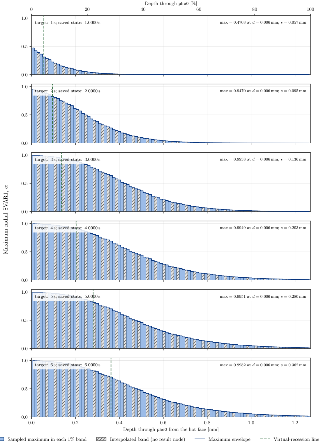
Figure 26. Evolution of radial SVAR1 profiles from 1 to 6 s. The recession line is shown in every panel.
