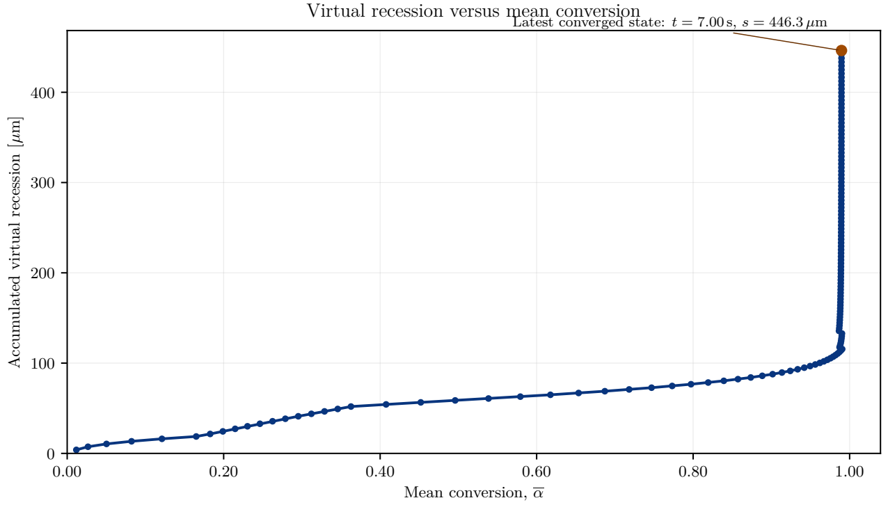
Figure 23. Accumulated virtual recession versus active-layer mean conversion.
