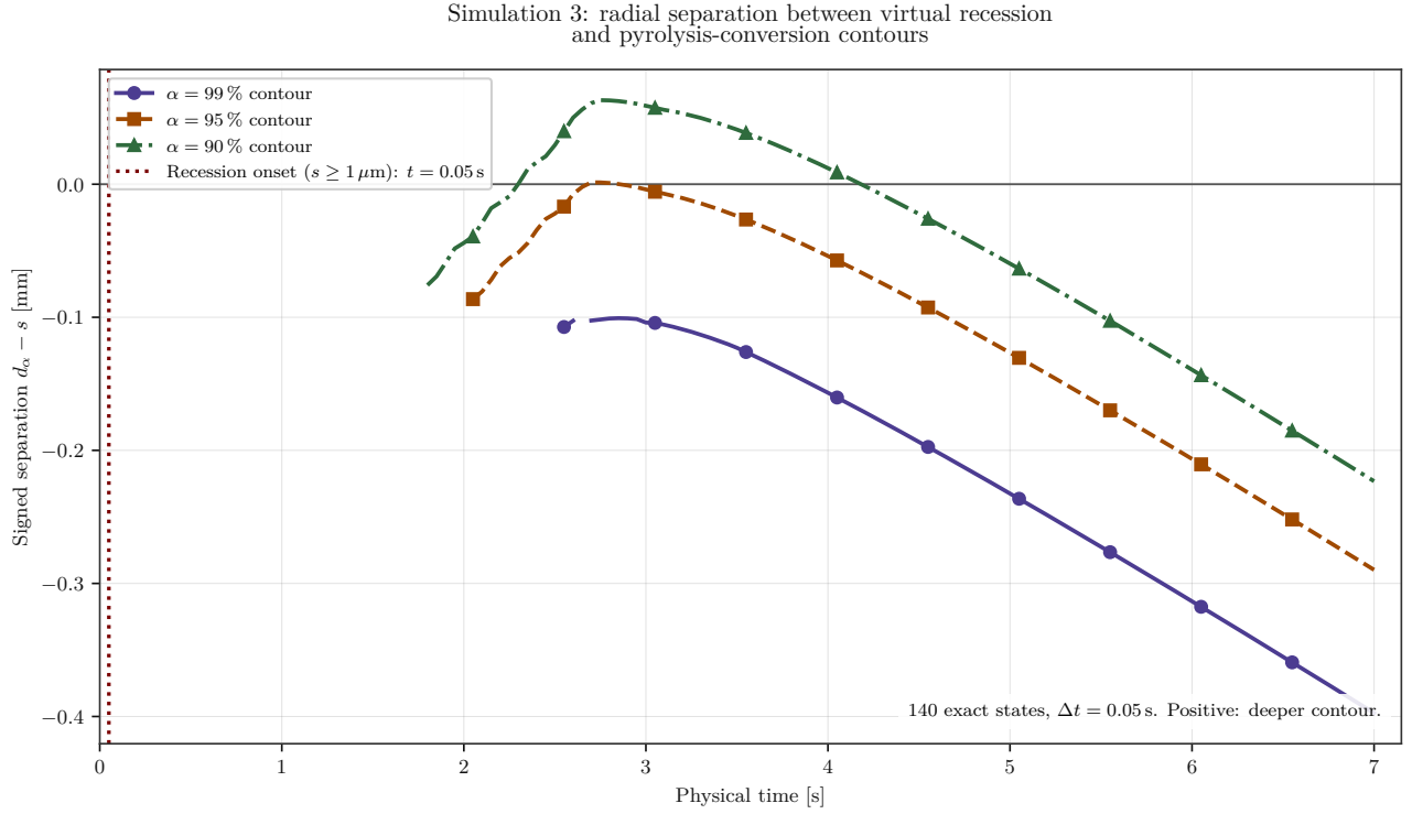
Figure 30. Signed separation between the recession line and the 99%, 95%, and 90% conversion contours over all 140 states. Positive values place the contour deeper into the wall. The vertical line marks the first numerically significant recession.
