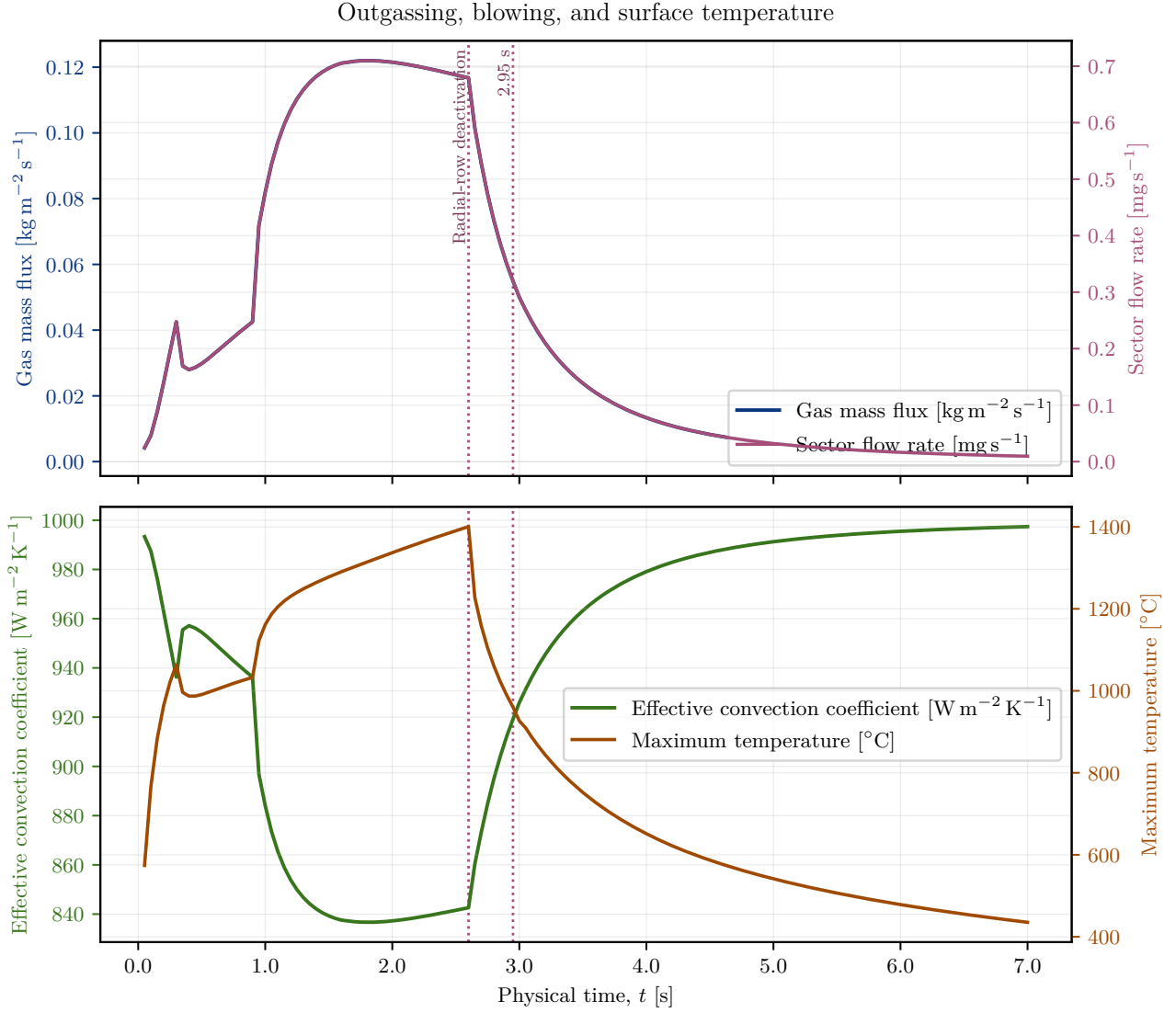
Figure 20. Evolution of outgassing, effective convection coefficient, and maximum hot-surface temperature. Total flow is for the 0.10^\circ sector.
