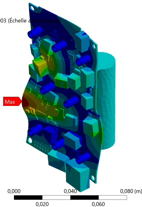
Figure 3: Six bolts at 750 N, rank 20: 2364.179 Hz. The PCB bends between the fixed stand-off locations, with coupled battery motion. This is an automatically scaled, mass-normalized mode shape; the legend is not a physical travel prediction.
