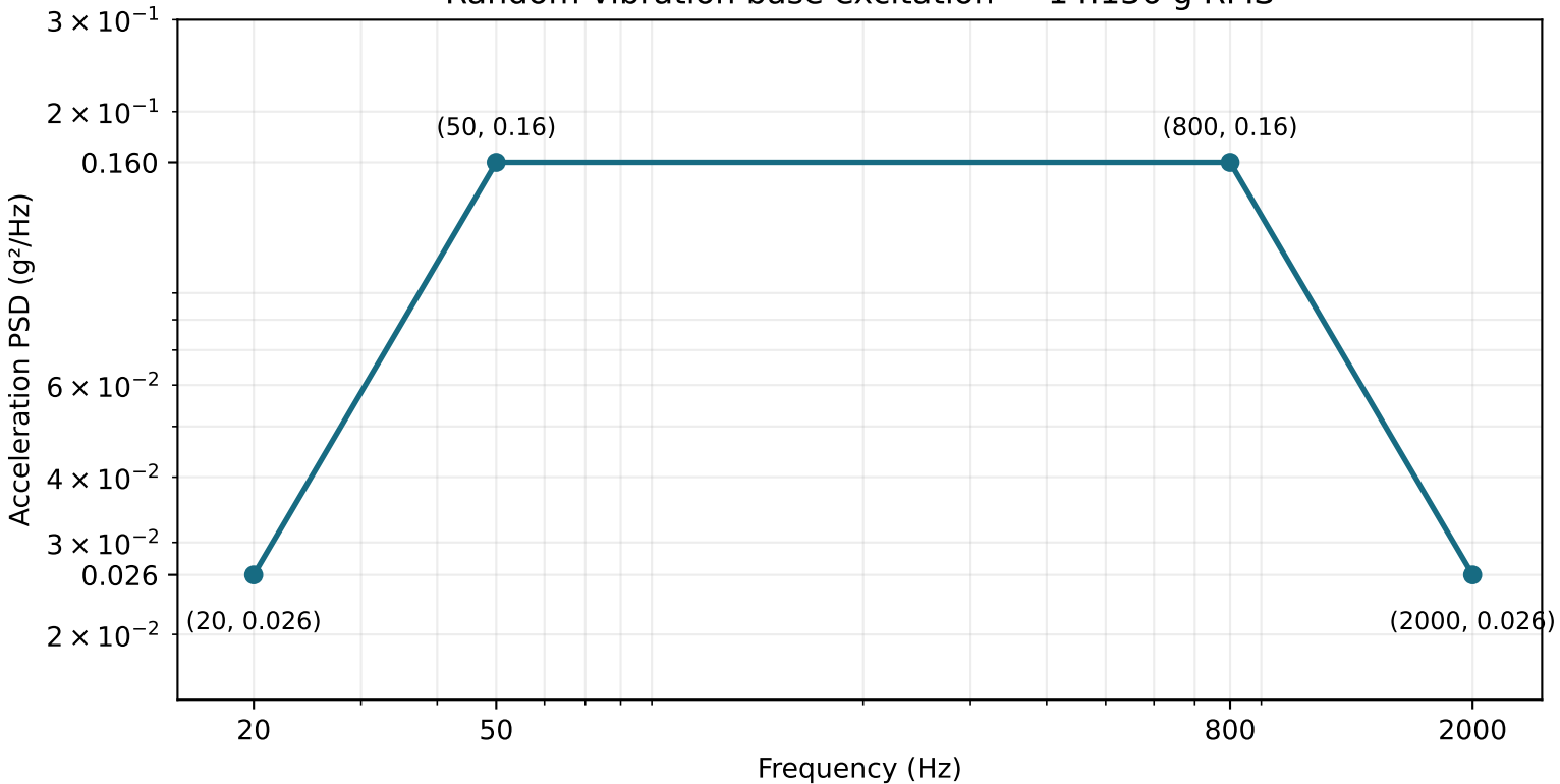
Random-vibration base excitation — 14.136 g RMS
