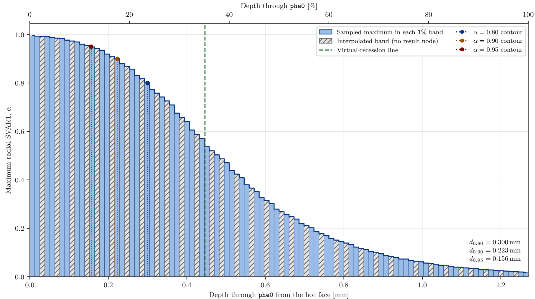
Simulation 3: radial SVAR1 profile at the final extracted state t = 7.0000 s; recession line s = 0.446 mm
