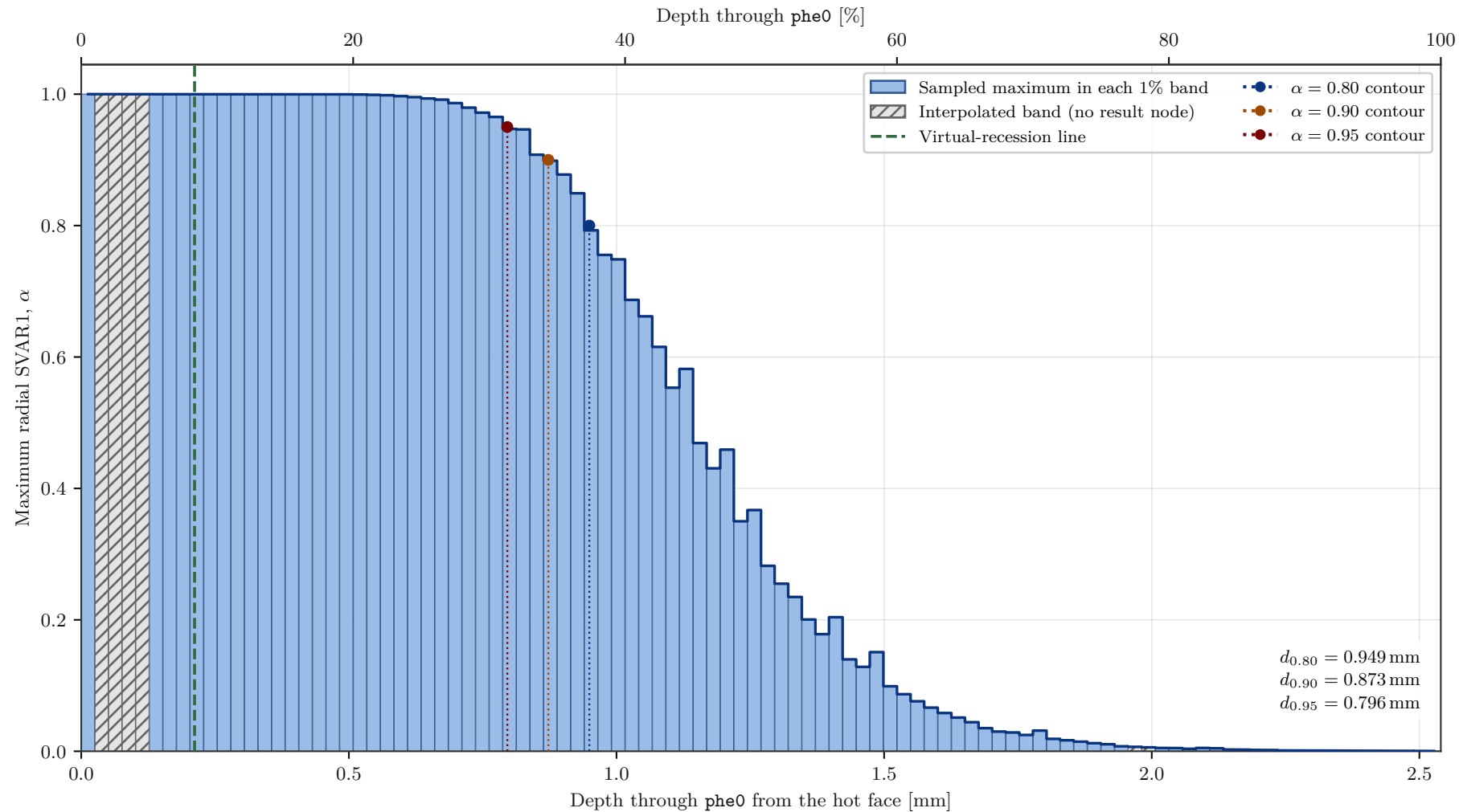
Simulation 2: radial SVAR1 profile at the latest extracted state t = 6.4500 s; recession line s = 0.212 mm
