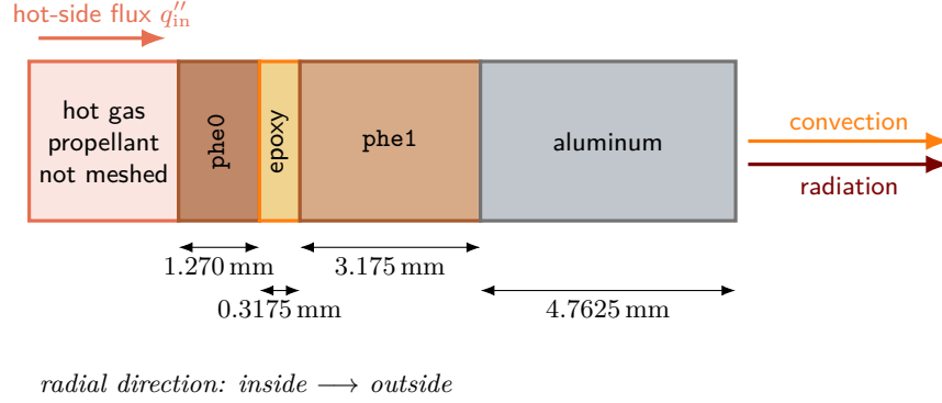
Figure 1. Corrected nominal radial layup. Layer widths are schematic; the stated dimensions are radial thicknesses.
