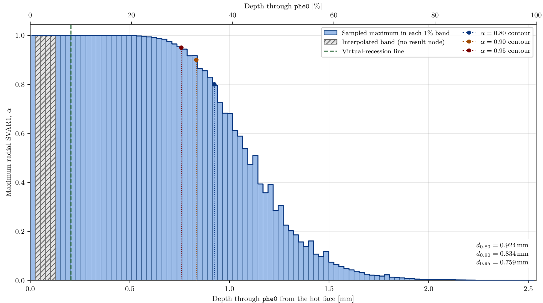
Simulation 2: radial SVAR1 profile at the latest extracted state t = 6.1500 s; recession line s = 0.204 mm
