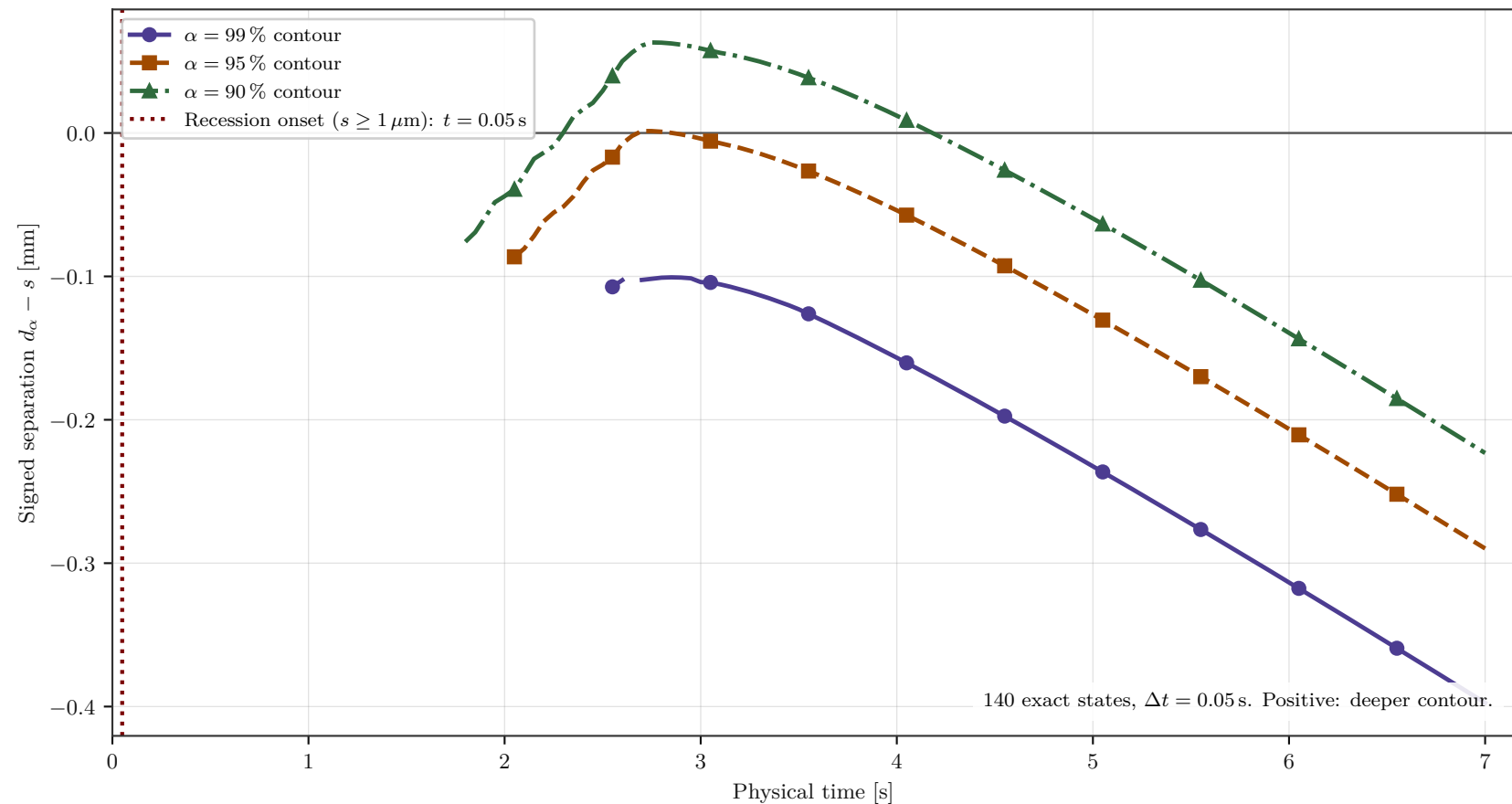
Simulation 3: radial separation between virtual recession and pyrolysis-conversion contours
