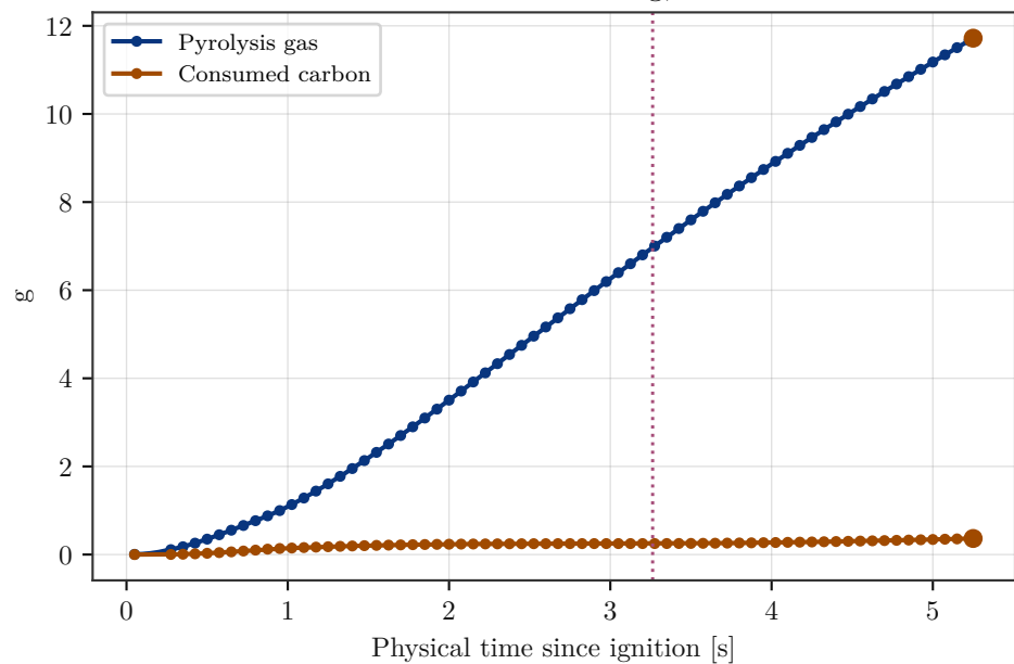
Cumulative masses: full ring, L = 50 mm
