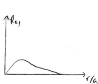
(e) n_r = 0, l = 1, n = 2
