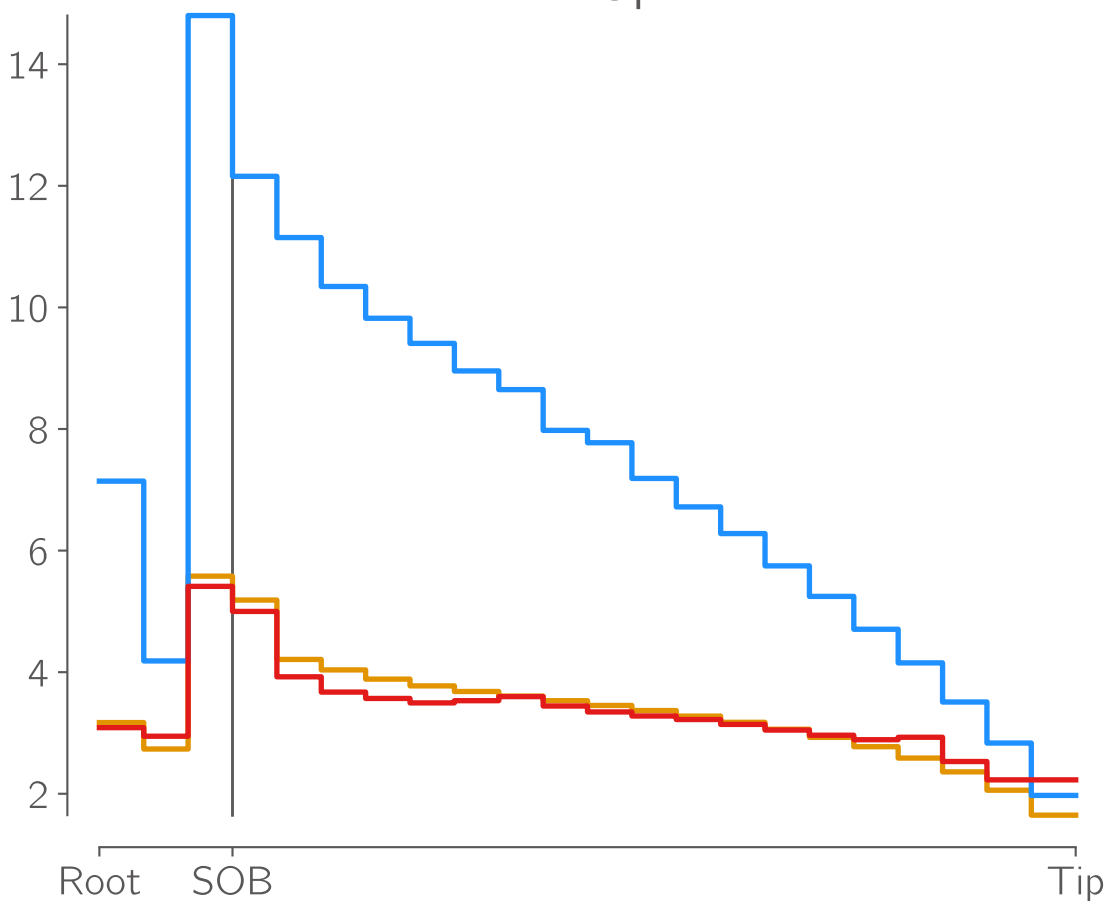
Rear Spar
