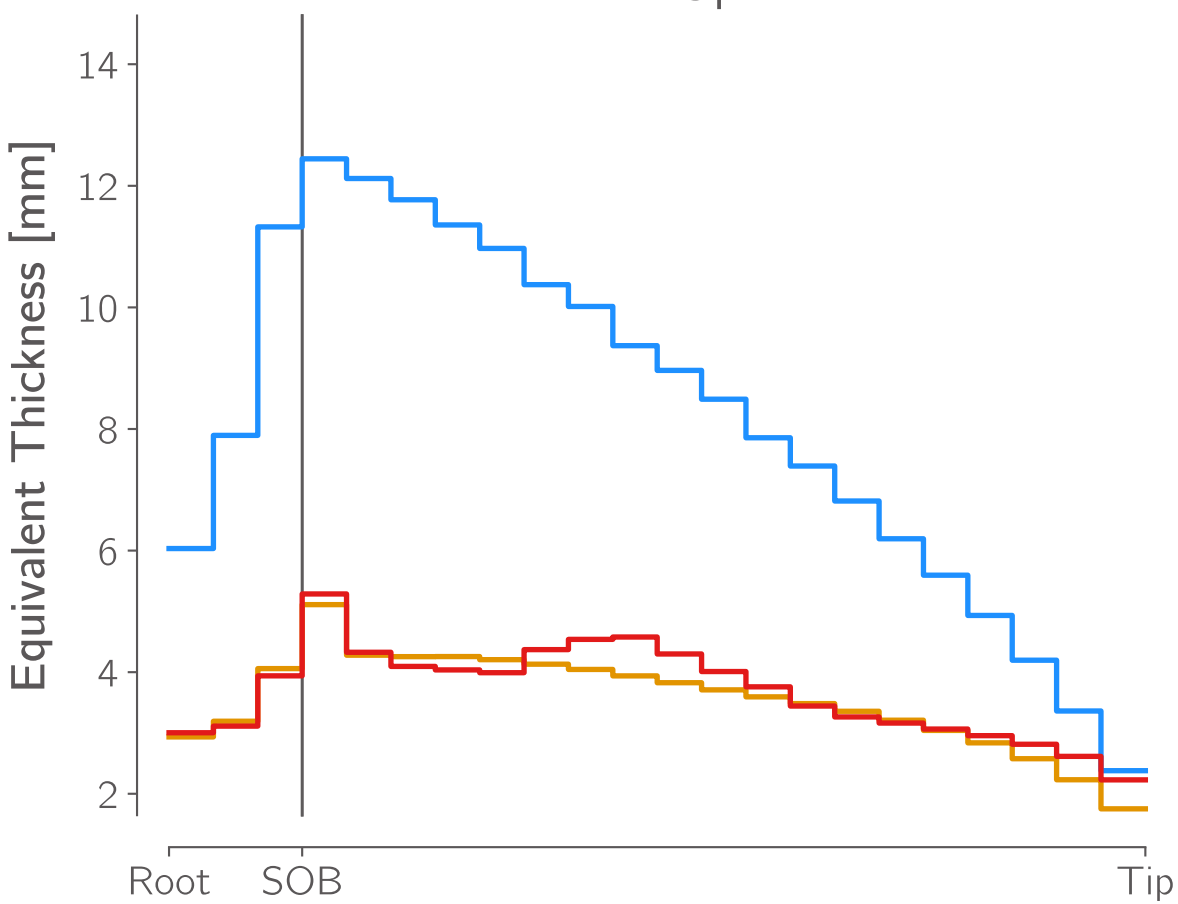
Front Spar
