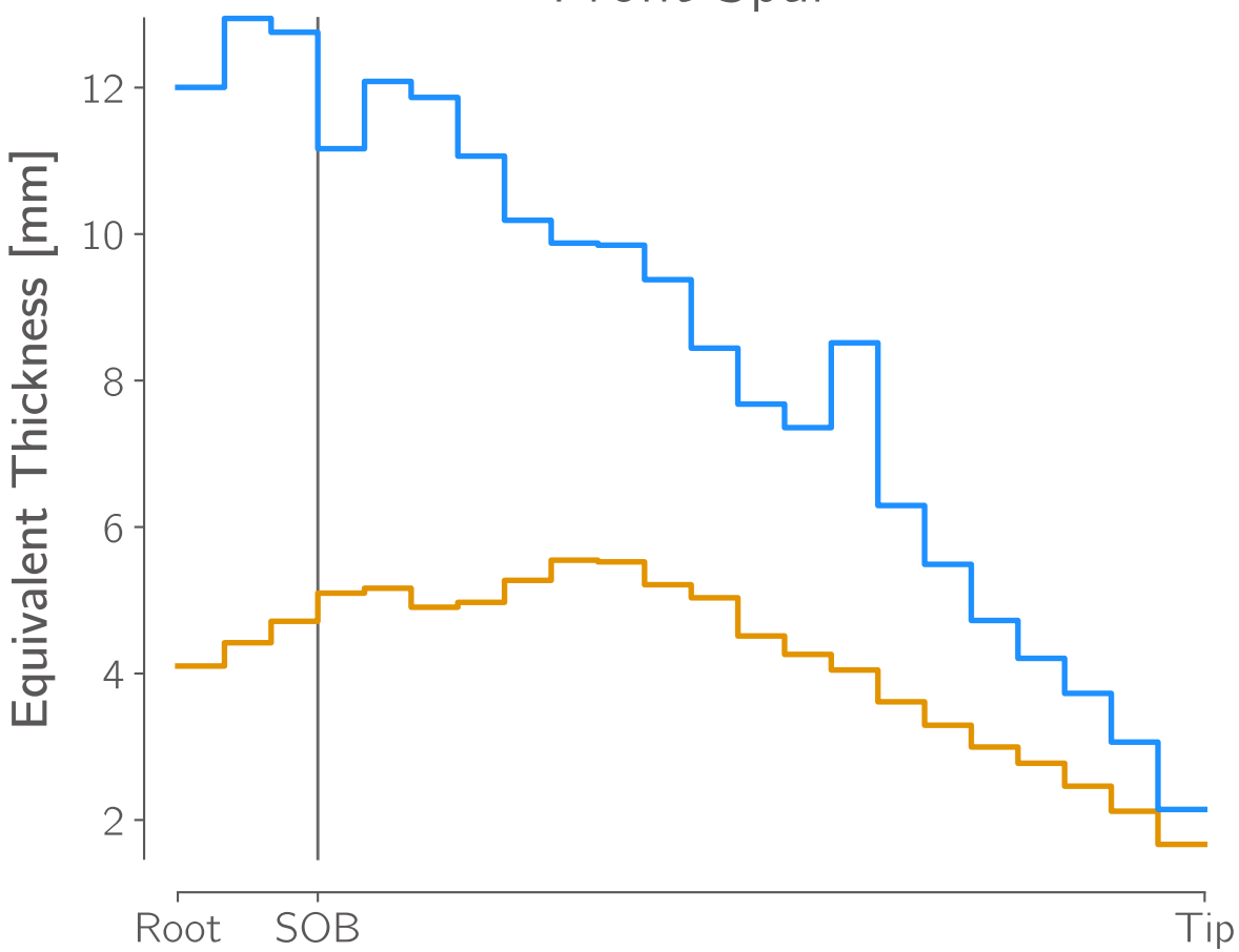
Front Spar
