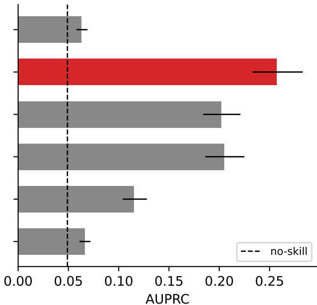
Discrimination: organ-decomposed matches/beats monolithic test (internal) external (CVICU)
