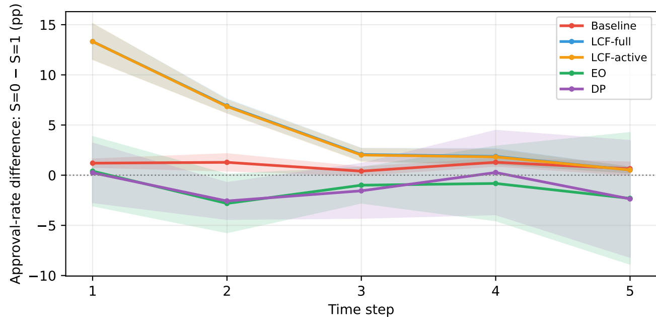
Variant II — mean \pm SD across 5 evaluation seeds Approval-rate difference \cdot base 80/20 \cdot opt-out enabled
