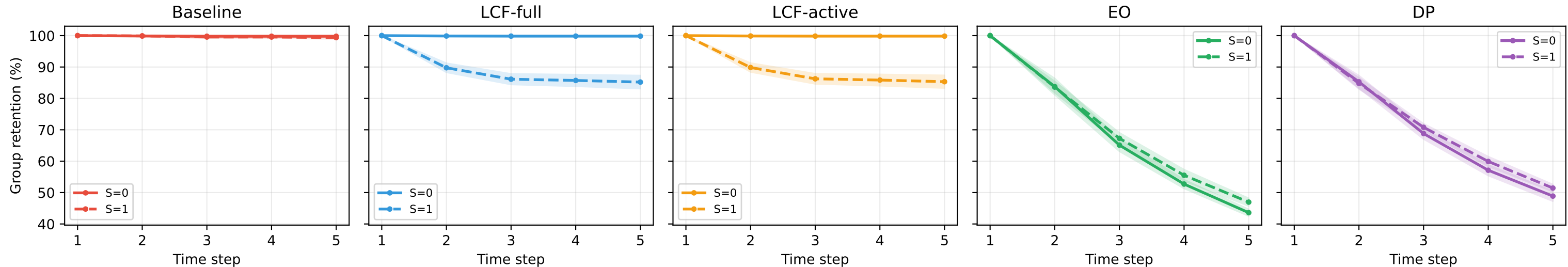
Variant II — mean \pm SD across 5 evaluation seeds Group retention · base 80/20 · opt-out enabled
