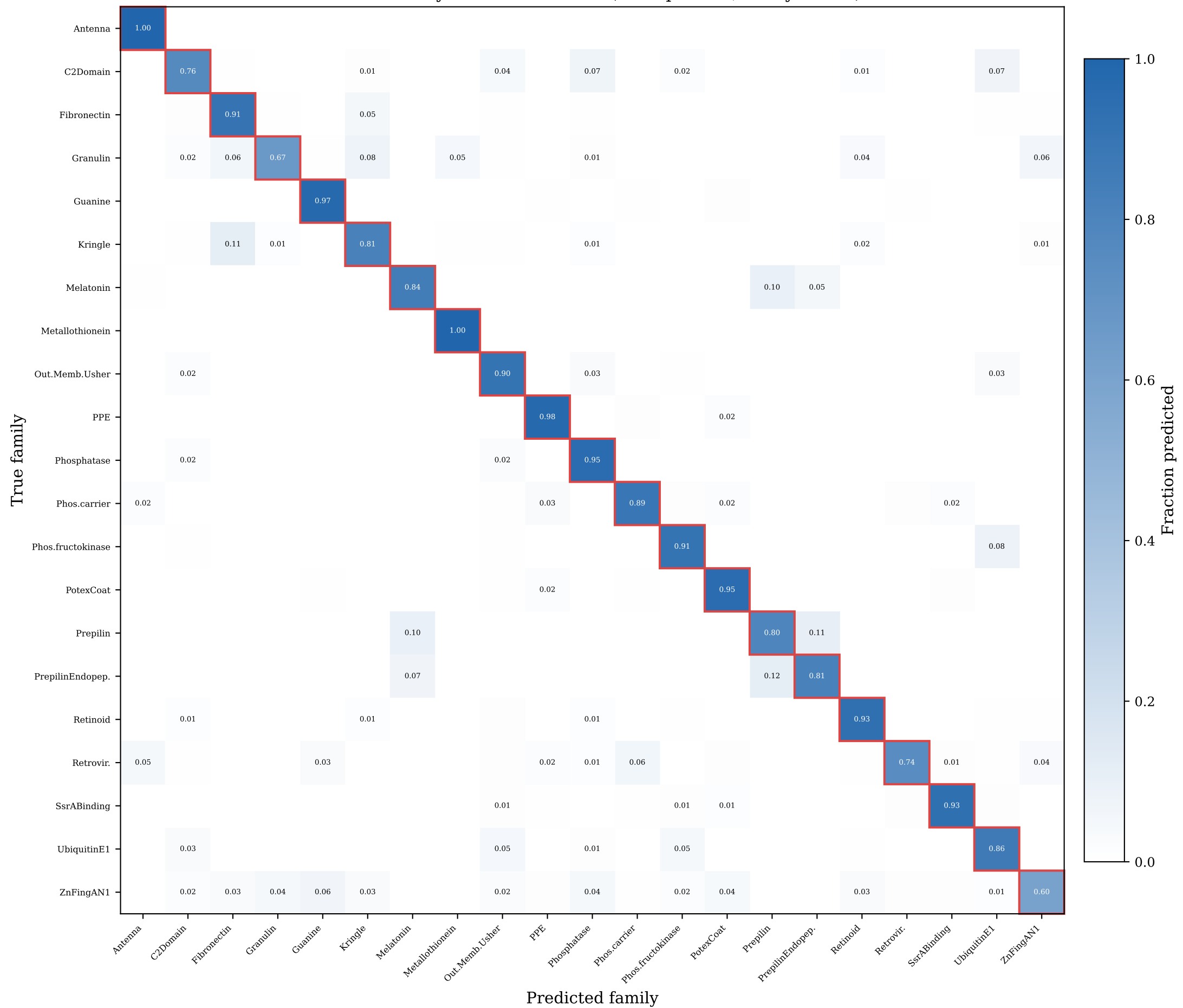
Named family confusion matrix (300 episodes, 5-way 5-shot)
