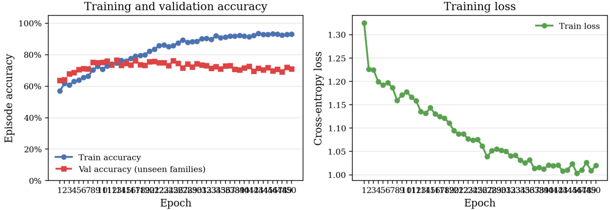
Figure 2: Training loss (right) and episode-level accuracy (left) per epoch on the 155-family dataset (124 training / 31 validation families), trained for 50 epochs with cosine-annealing LR ( T_{\max} = 50 ). Training accuracy rises from 57.3% (epoch 1) to 93.1% (epoch 50). Validation accuracy peaks at 76.6% at epoch 13, then gradually declines—a delayed form of task-distribution overfitting compared to the 21-family setting (epoch 3). The best checkpoint (epoch 13, val_acc = 0.766) is used for all S2 evaluation.
