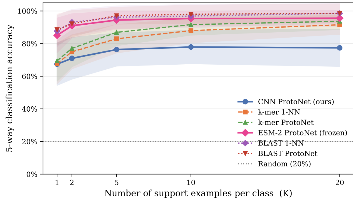
Few-shot accuracy vs. number of shots (5-way, cosine metric)
