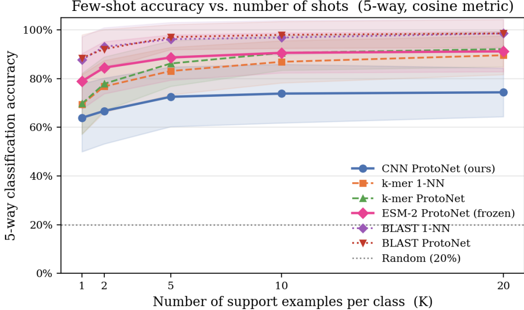
Figure 3: 5-way accuracy vs. number of support examples K for CNN ProtoNet (ours), k-mer 1-NN, and k-mer ProtoNet on the 24 held-out test families (S2), including the frozen ESM-2 ProtoNet. Shaded bands show \pm 1\sigma . ESM-2 leads at K \leq 5 (up to +9.9 pp over k-mer); k-mer ProtoNet closes the gap from K = 5 onward and edges ESM-2 at K = 20 (91.7% vs 91.2%). CNN ProtoNet remains ~15–18 pp below k-mer across all K .
