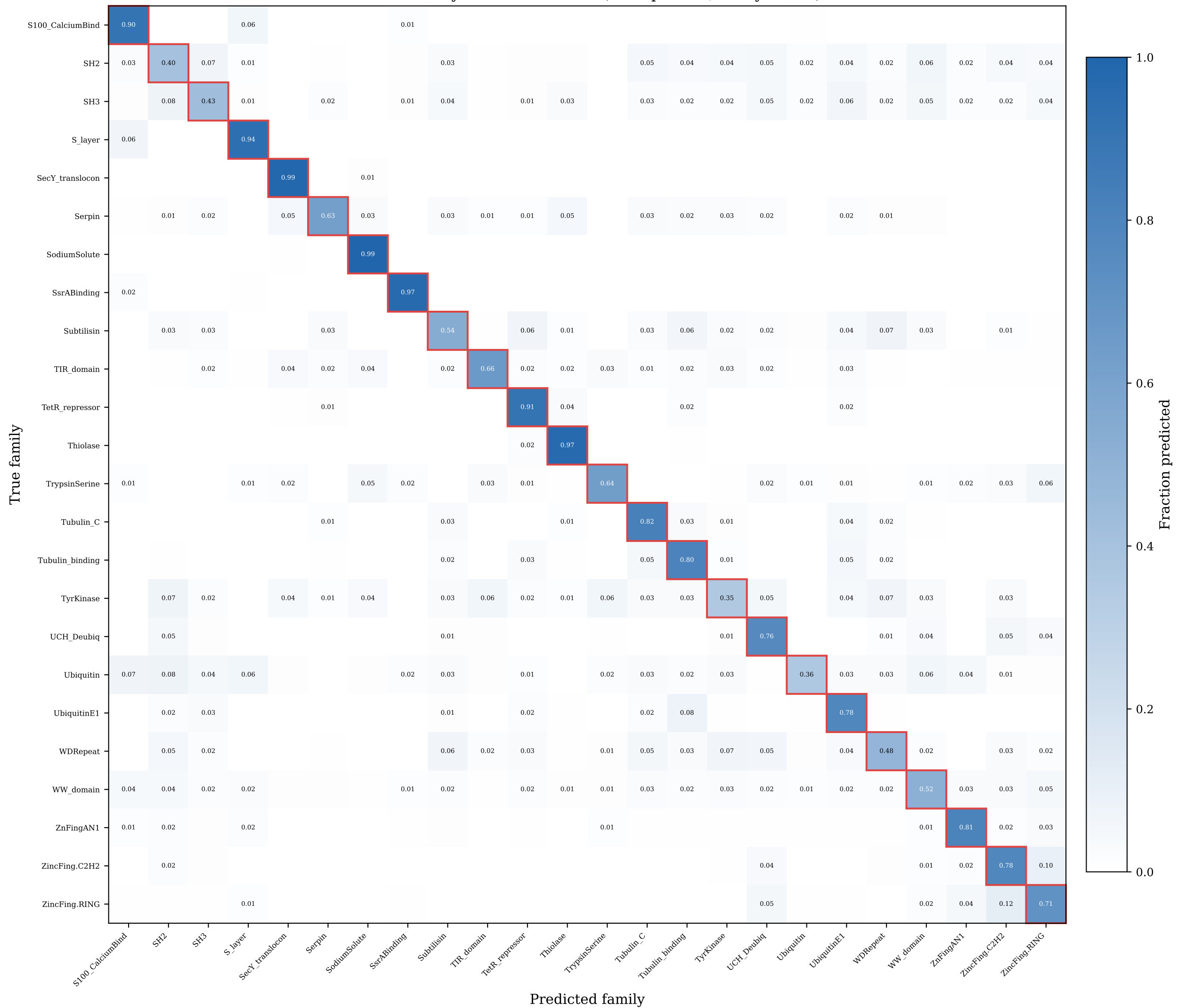
Named family confusion matrix (300 episodes, 5-way 5-shot)
