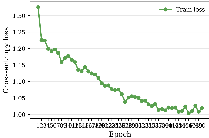
Training loss
