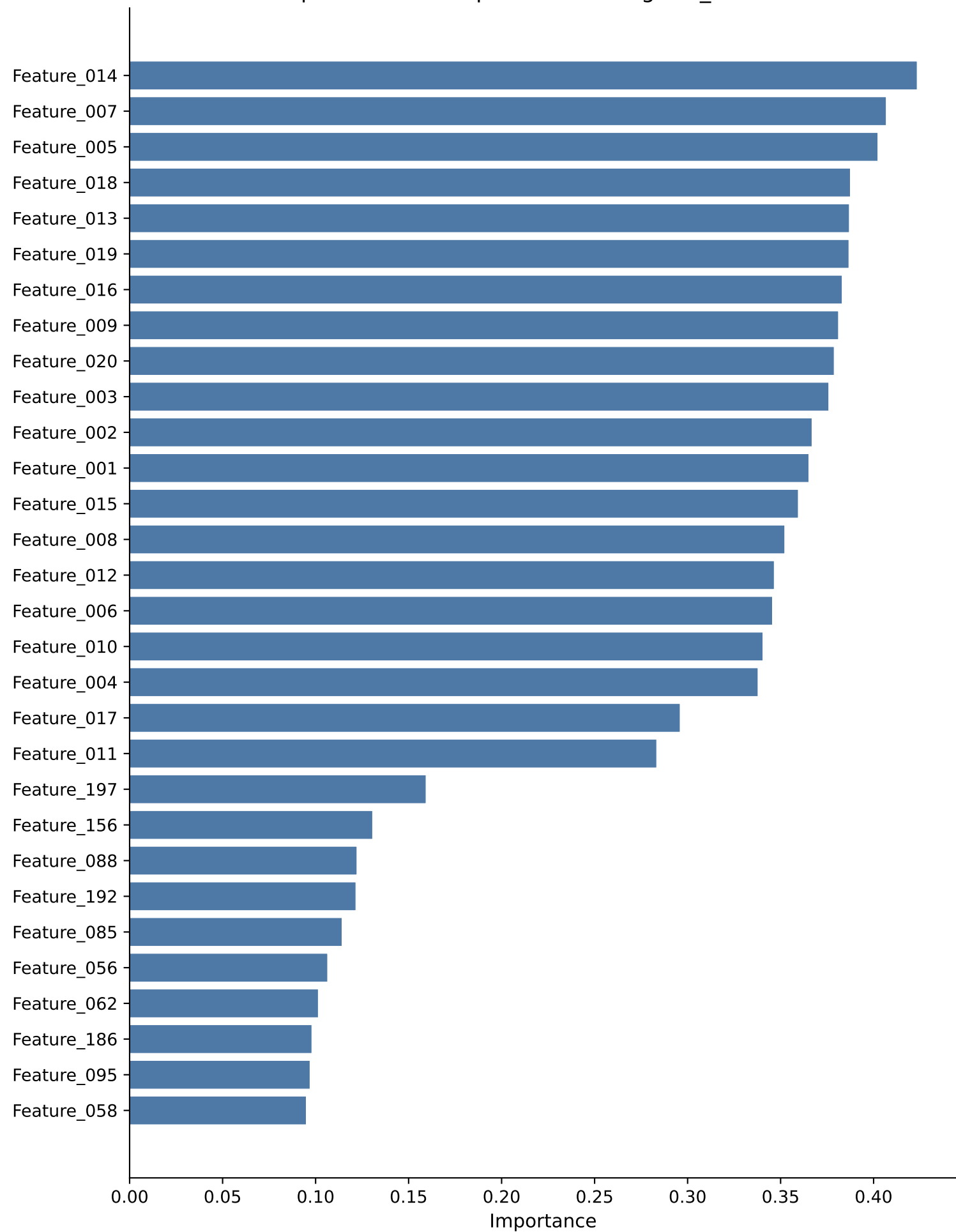
Top 30 Feature Importances · logistic_classifier
