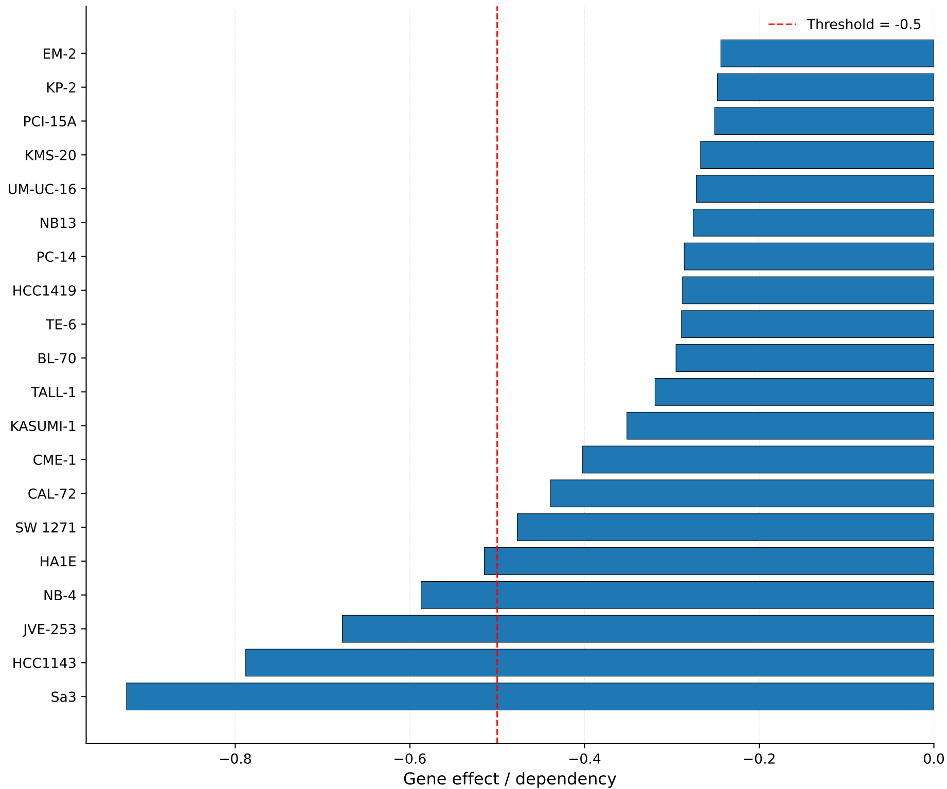
TP53 most dependent cell lines
