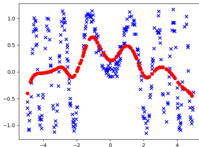
Figure 3: Locally weighted linear regression with \tau = 0.5 on the 'train' split. (MSE: 0.330531268213752)
