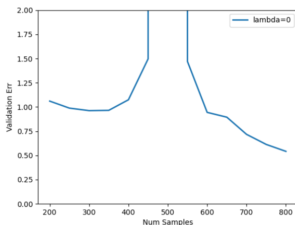
Figure 11: Double Descent phenomenon on different sample sizes
