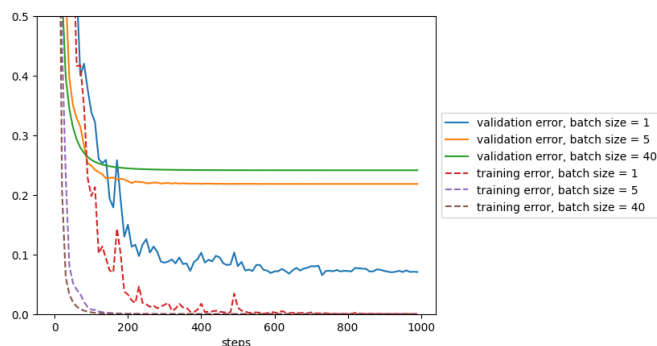
Figure 10: Validation loss with different batch sizes
