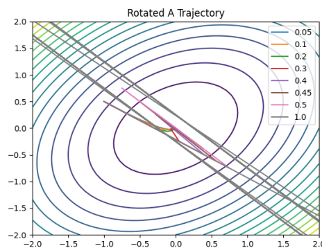
Figure 2: Gradient descent trajectories with rotated A .
