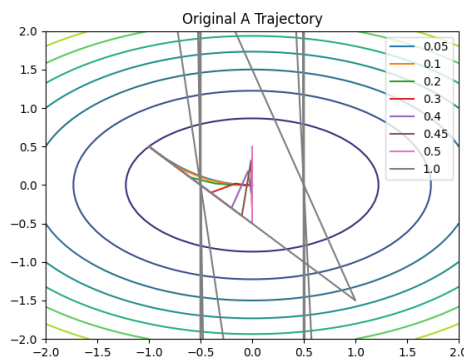
Figure 1: Gradient descent trajectories with regular A .
