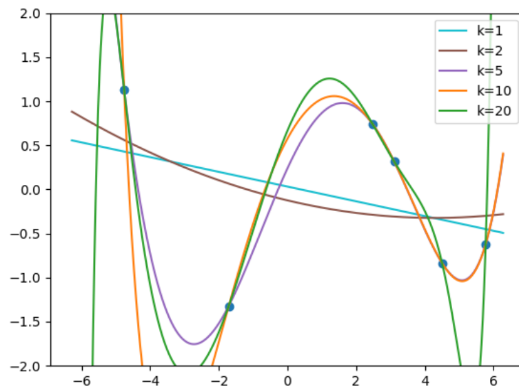
Figure 7: Polynomial regression with sine features
