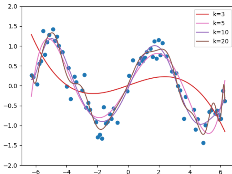
Figure 5: Polynomial regression with multiple degrees
