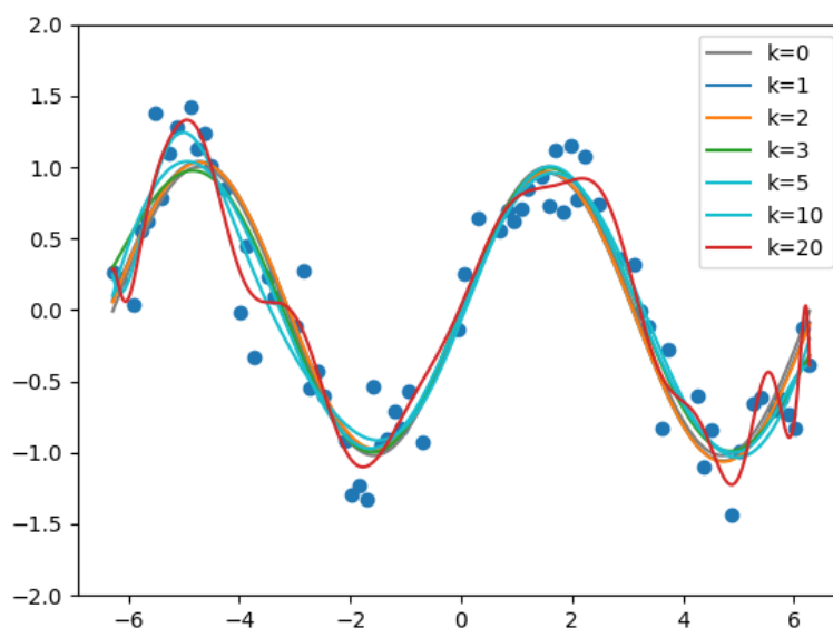
Figure 6: Polynomial regression with sine features
