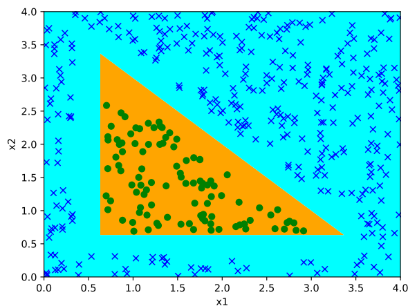
Figure 12: Decision Boundary – Step activations
