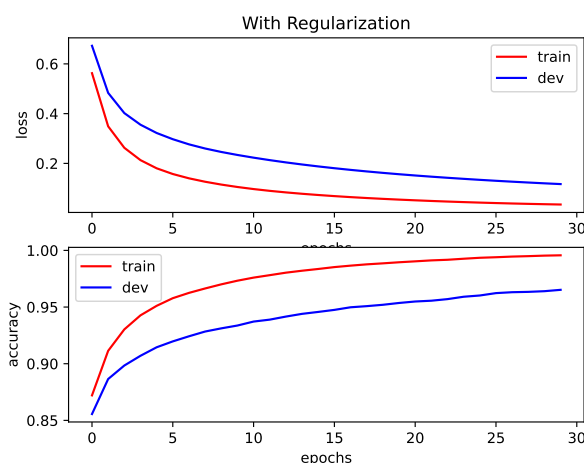
Figure 9: Accuracy & Loss vs. Epoch (Regularized Model)
