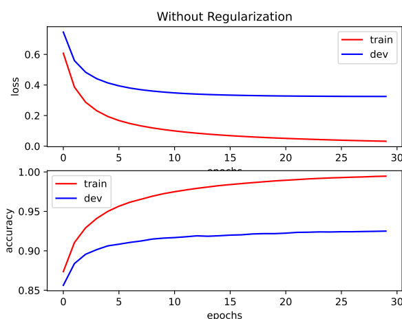
Figure 8: Accuracy & Loss vs. Epoch
