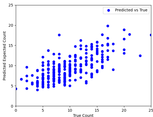
Figure 1: Poisson True vs. Predicted Values
