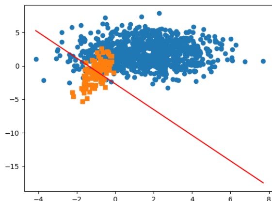
Figure 6: Vanilla Logistic Regression on imbalanced set
