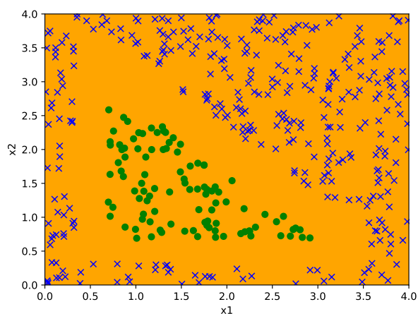
Figure 12: Decision Boundary – Linear Activations
