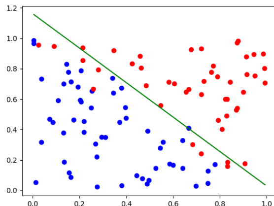
Figure 2: LR decision boundary dataset A
