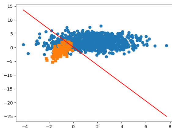
Figure 7: Reweighted Logistic Regression on imbalanced set
