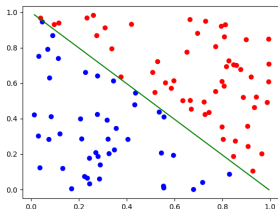
Figure 3: LR decision boundary for dataset B
