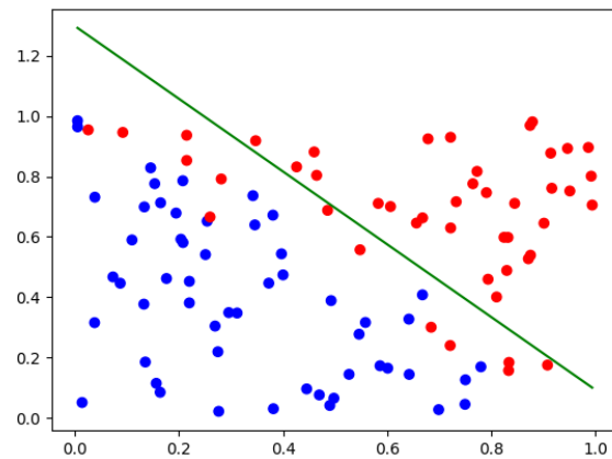
Figure 4: LR decision boundary for dataset A (Regularized)
