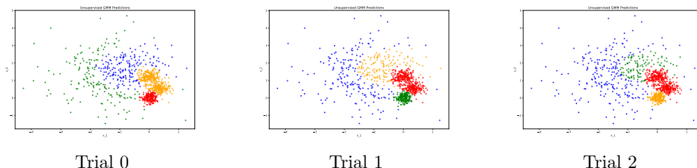
Figure 2: Results of unsupervised EM algorithm across three different trials with random initializations.
