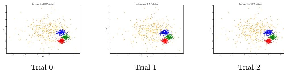
Figure 3: Results of semi-supervised EM algorithm across three different trials with random initializations.
