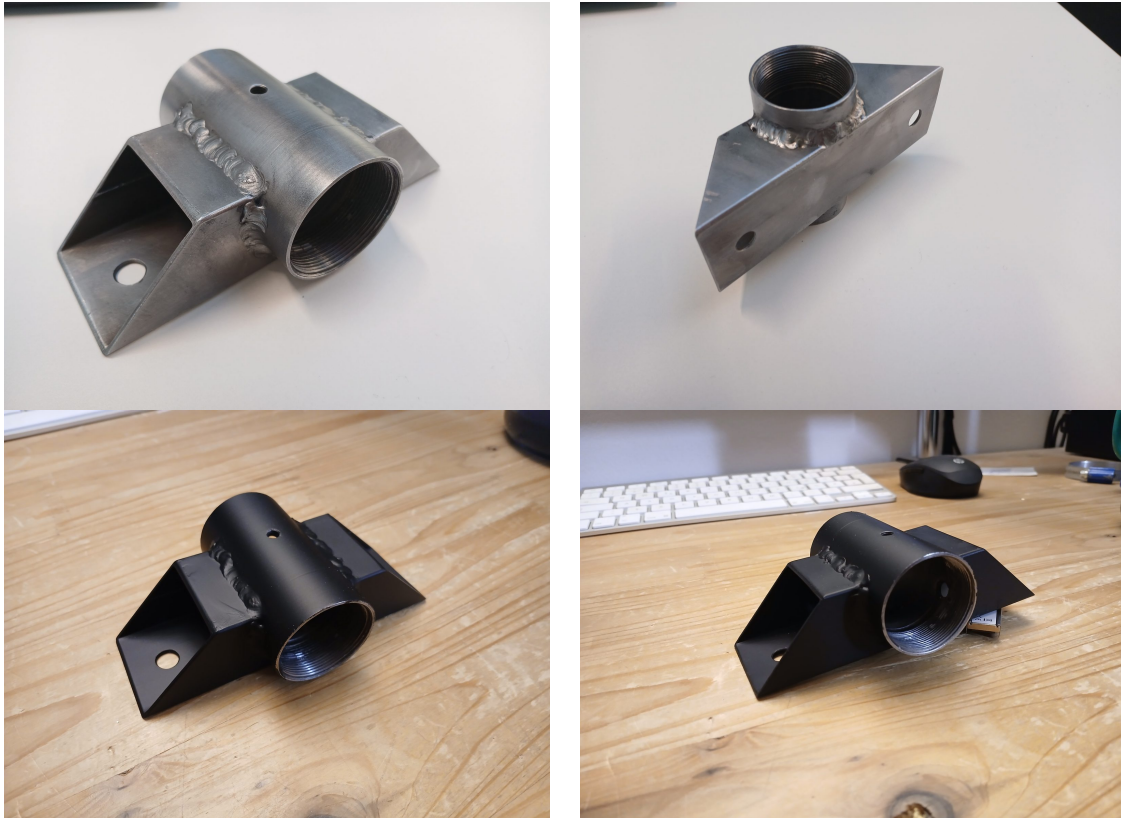
Figure 4.1: Bottom bracket shell manufacturing steps.
