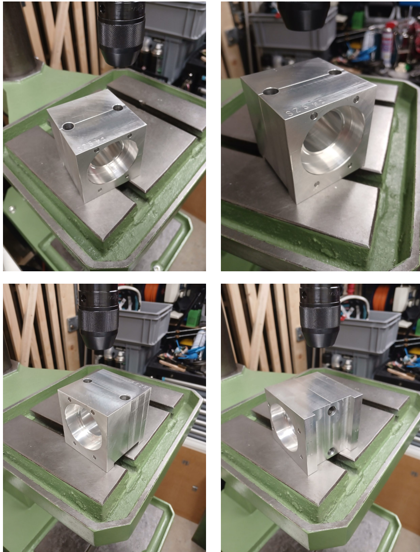
Figure 4.2: Pillow block manufacturing steps.
