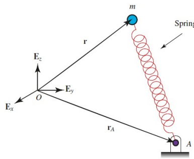
Figure 14.1: General spring configuration
