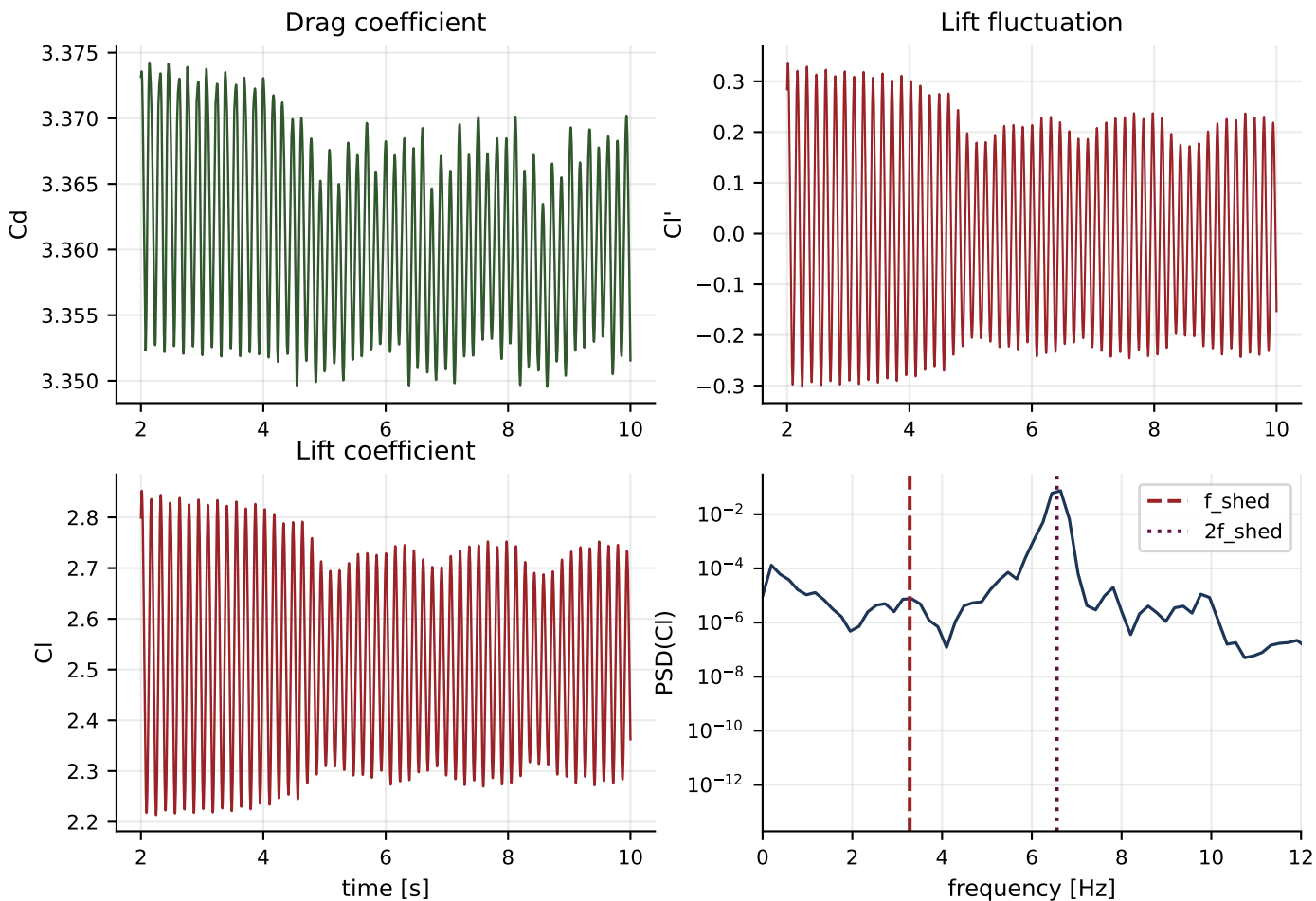
Figure 2. Force history and lift spectrum
