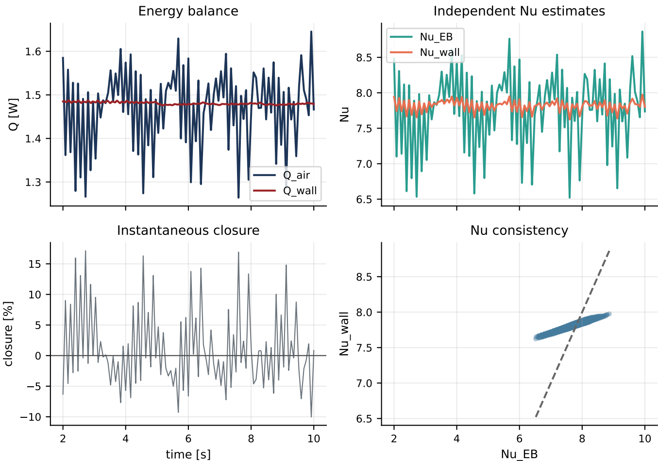
Figure 3. Heat balance and Nusselt closure
