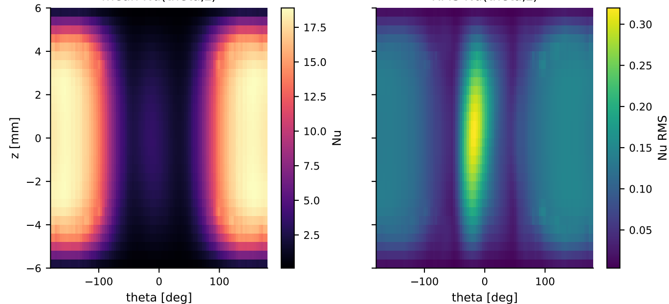
Figure 4. Tube local Nusselt statistics
