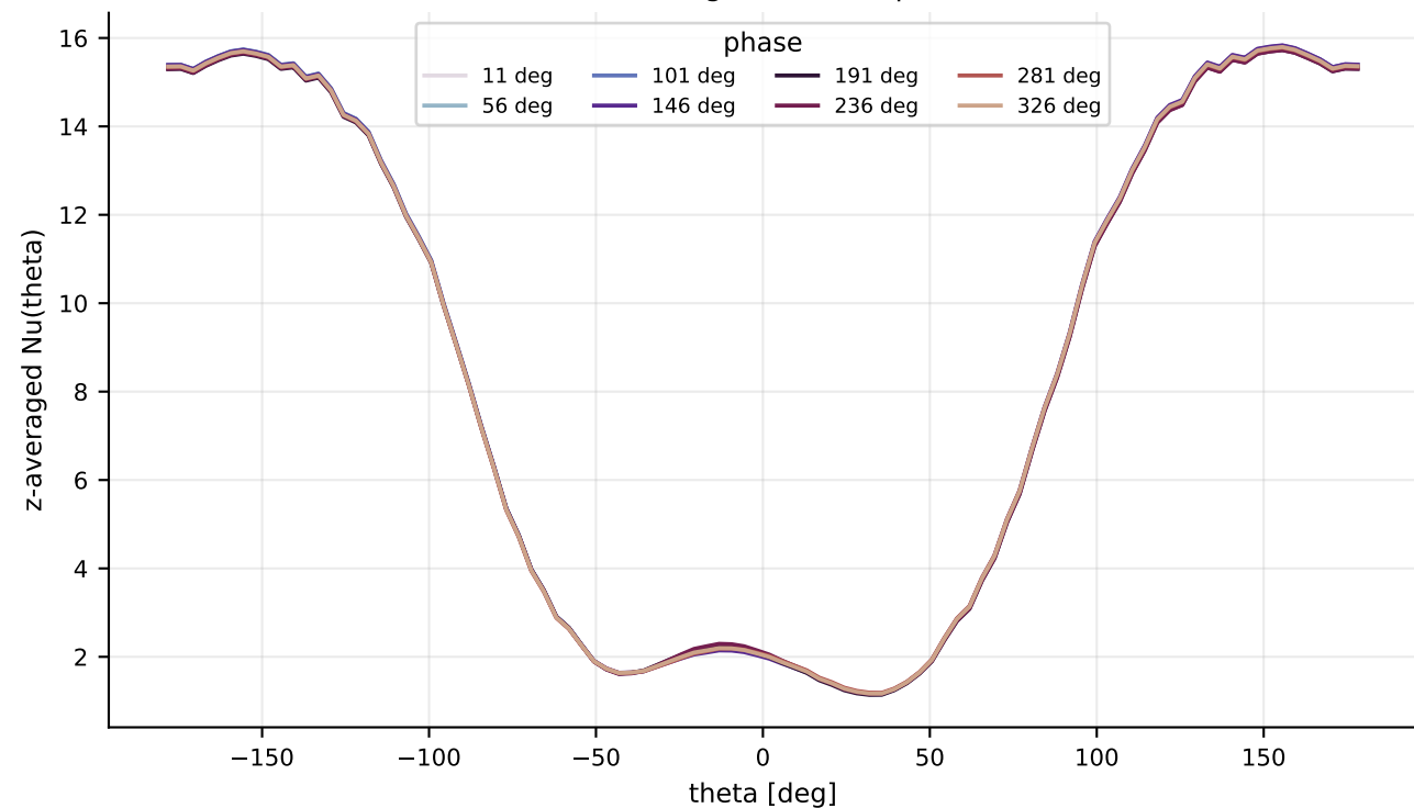
Figure 5. Phase-resolved Nu(theta)
