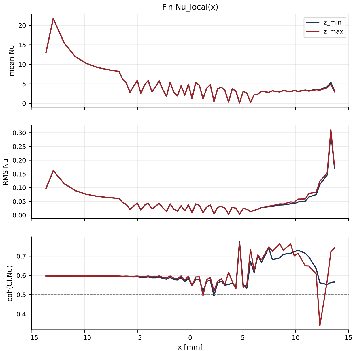
Figure 6. Fin local heat-transfer response
