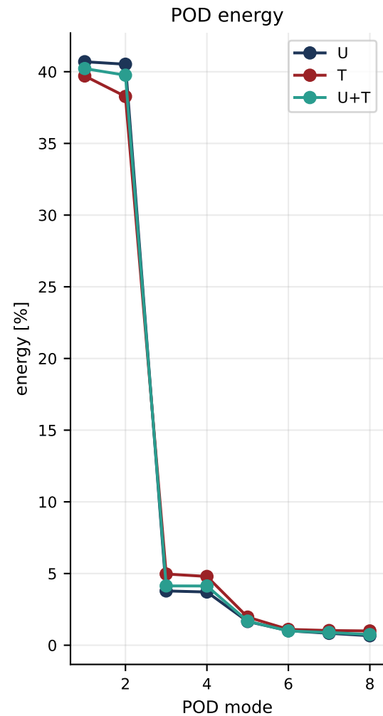
Figure 7. POD energy and dominant mode maps
