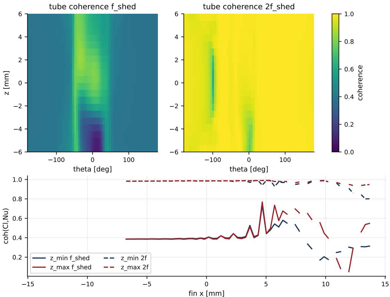
Figure 9. Coherence between lift and local Nu
