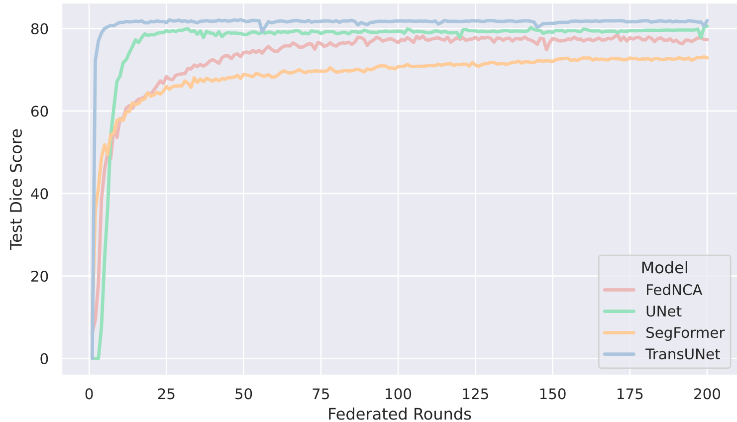
Convergence of Ultrasound Segmentation Models
