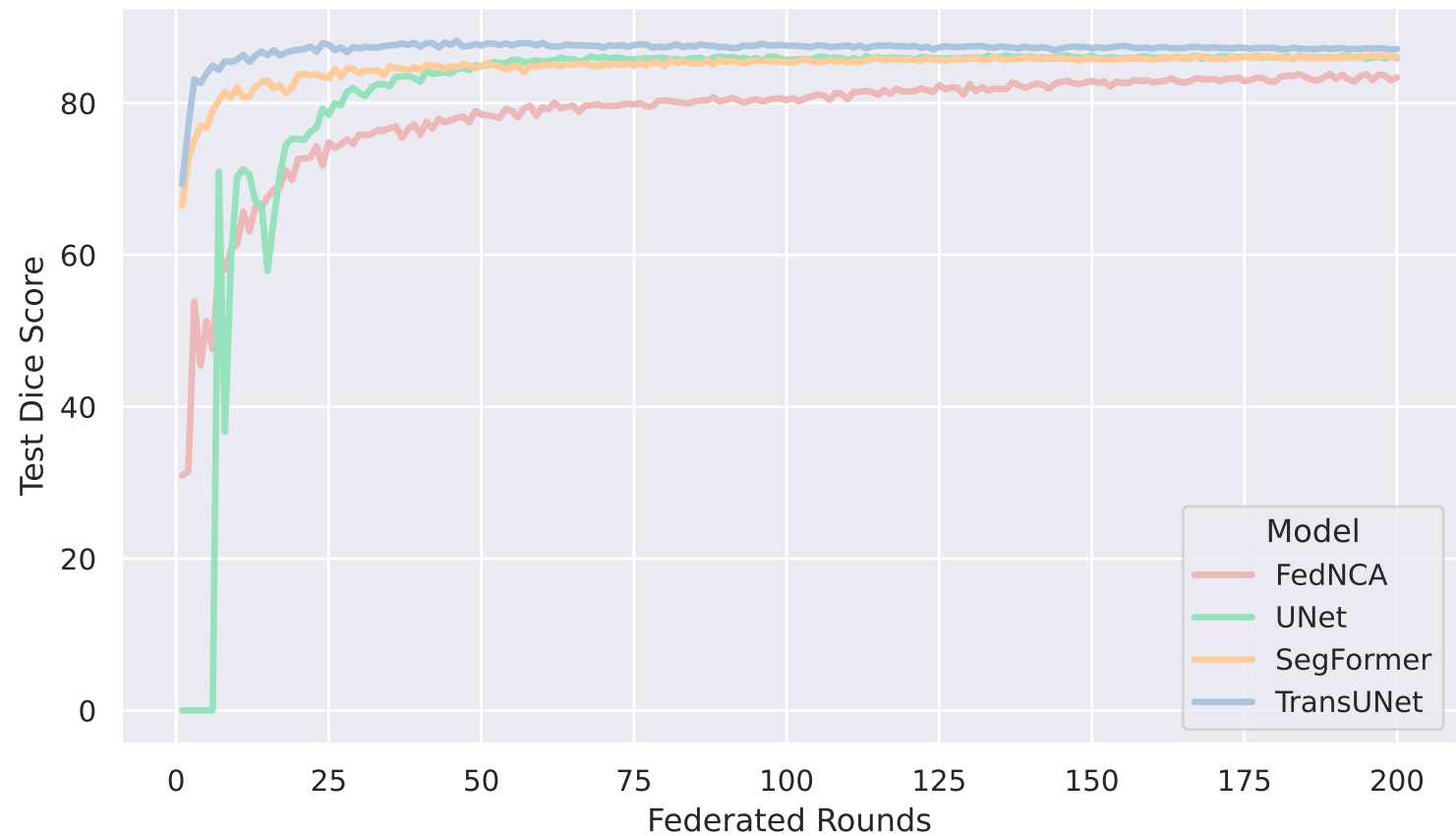
Convergence of XRay Segmentation Models
