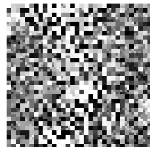
FedNCA (det)
