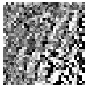
FedNCA
