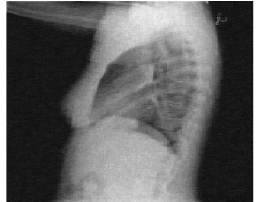
Unsupervised Cleaning
