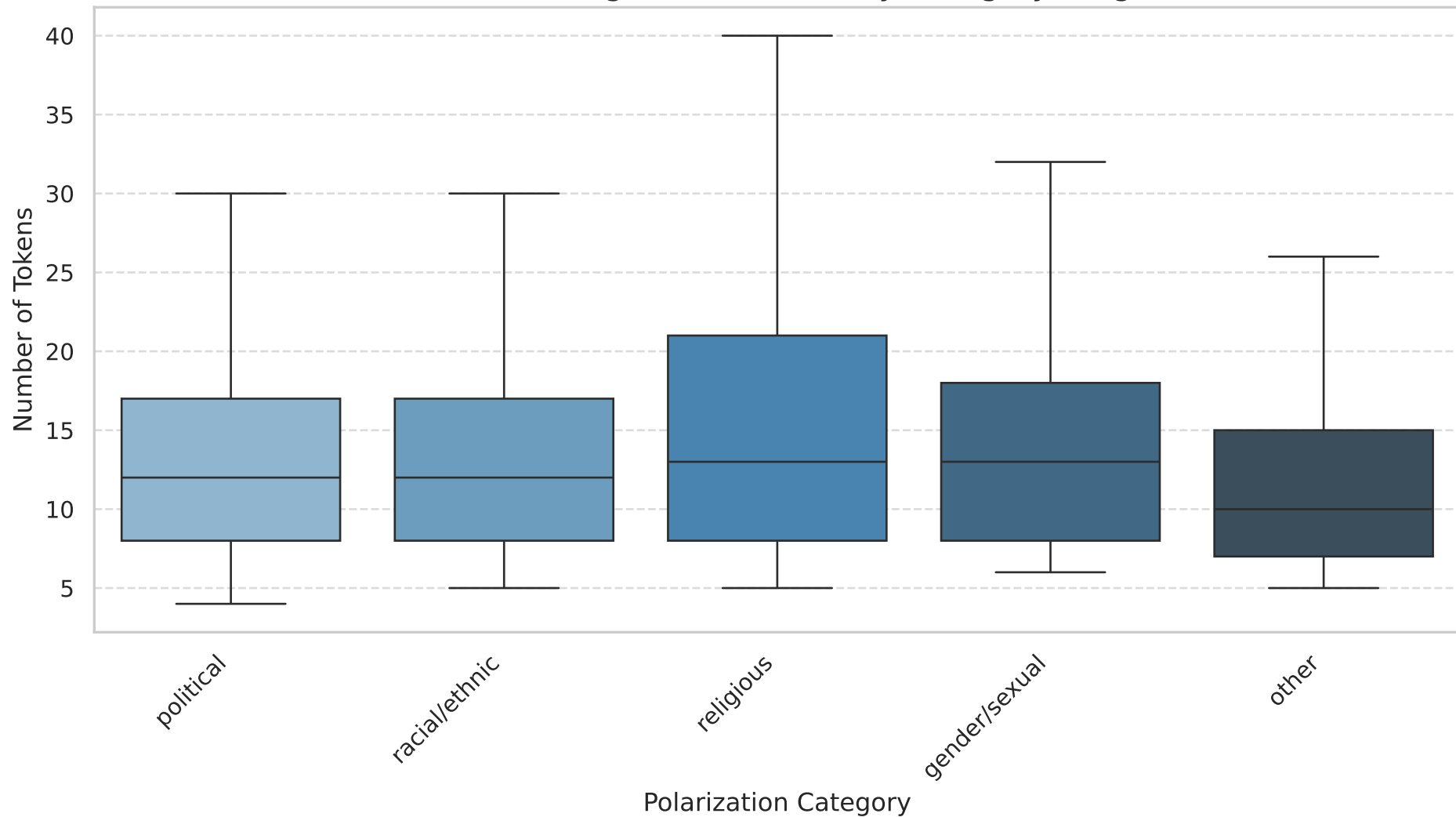
Task 2: Text Length Distribution by Category (English)
