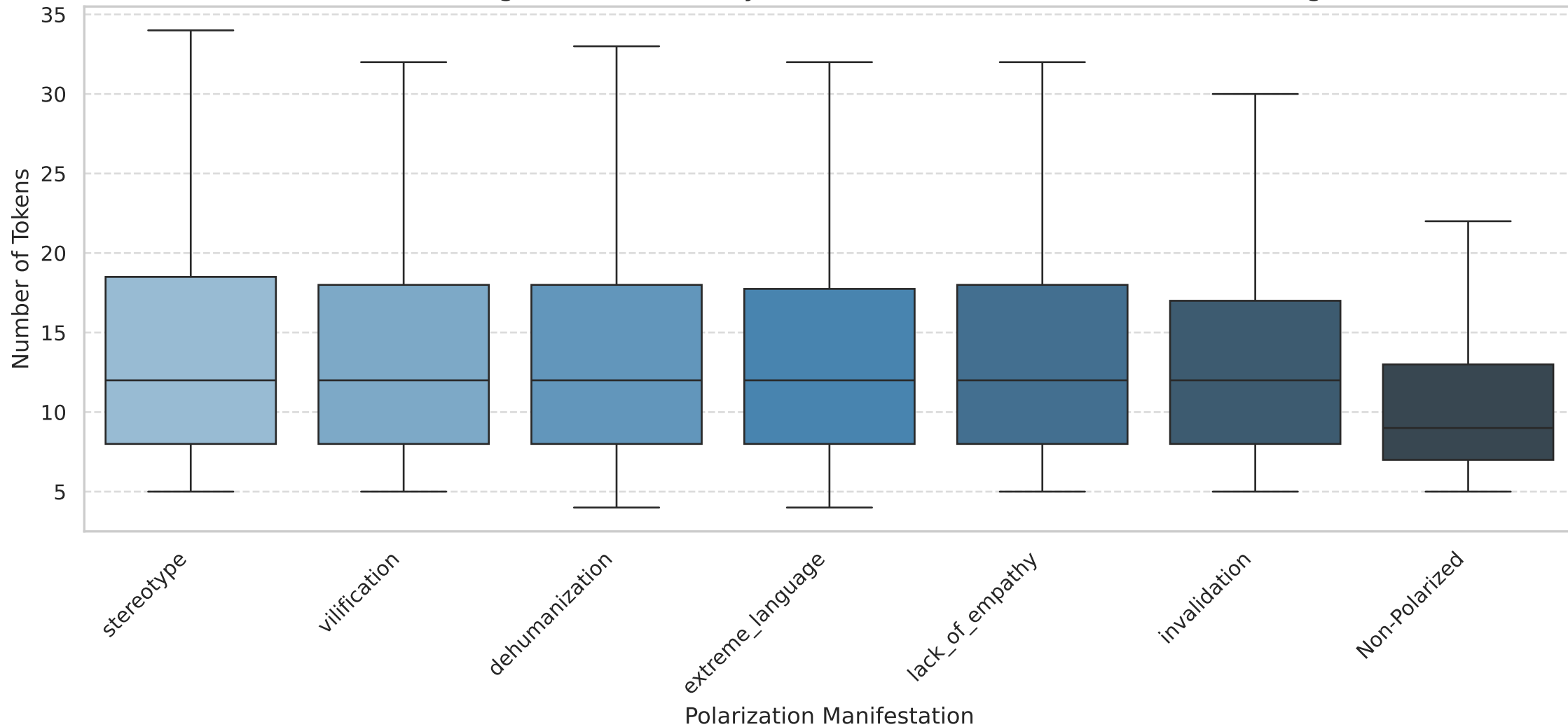
Task 3: Text Length Distribution by Manifestation (Incl. Non-Polarized) (English)
