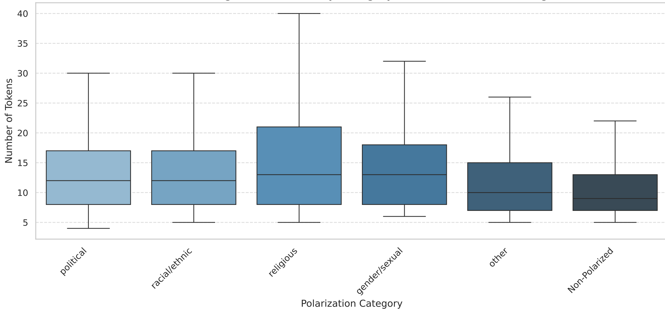
Task 2: Text Length Distribution by Category (Incl. Non-Polarized) (English)
