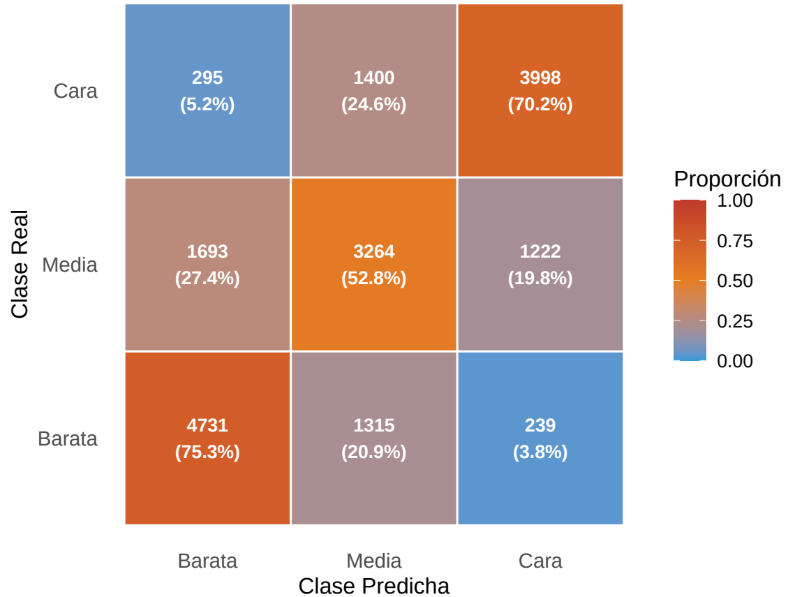
RNA-C2: Skip, 15 nodos
