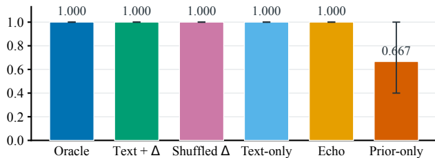
Preservation rate \uparrow
