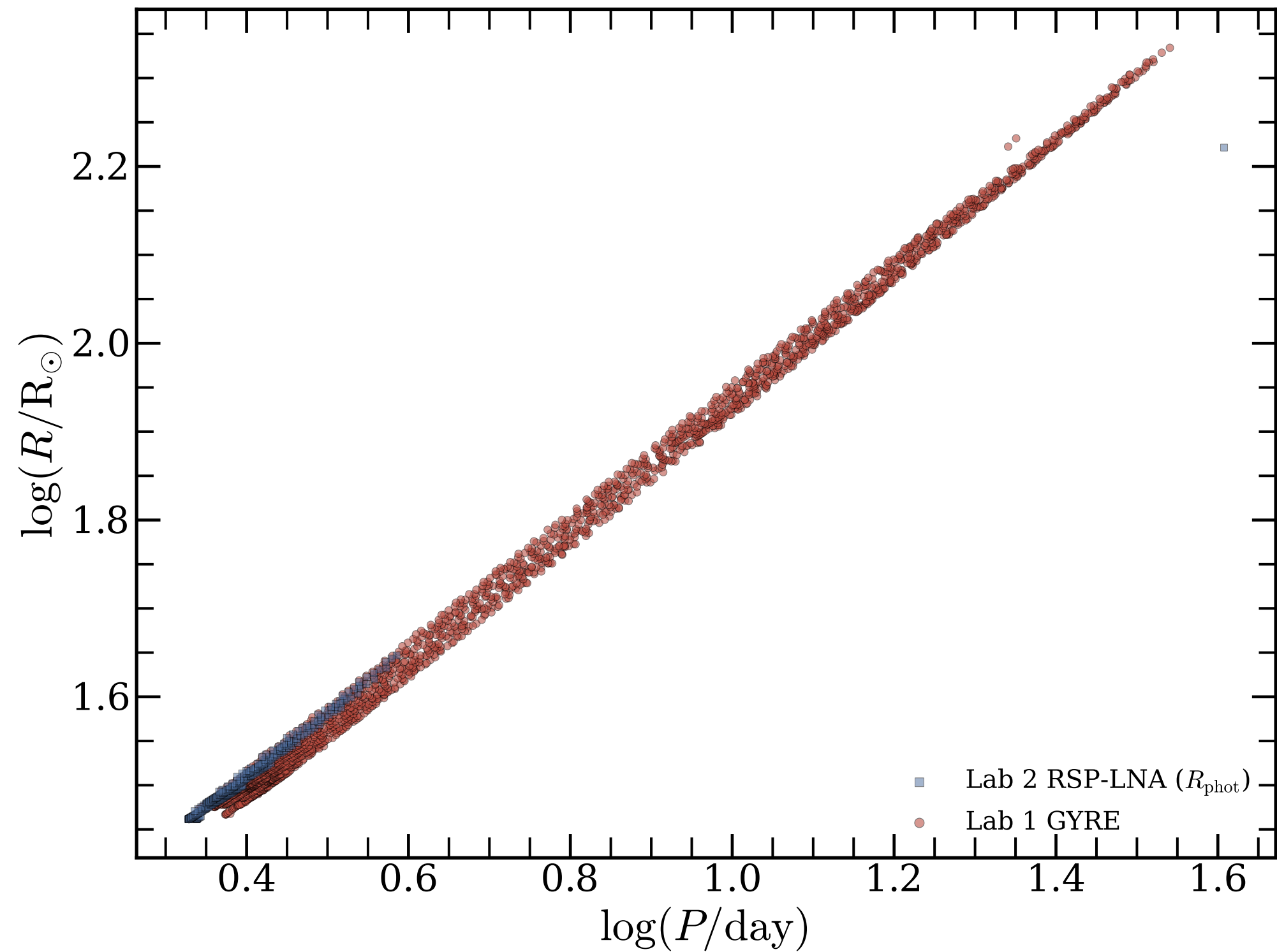
F_1 unstable, F_2 subdominant period-radius relation
