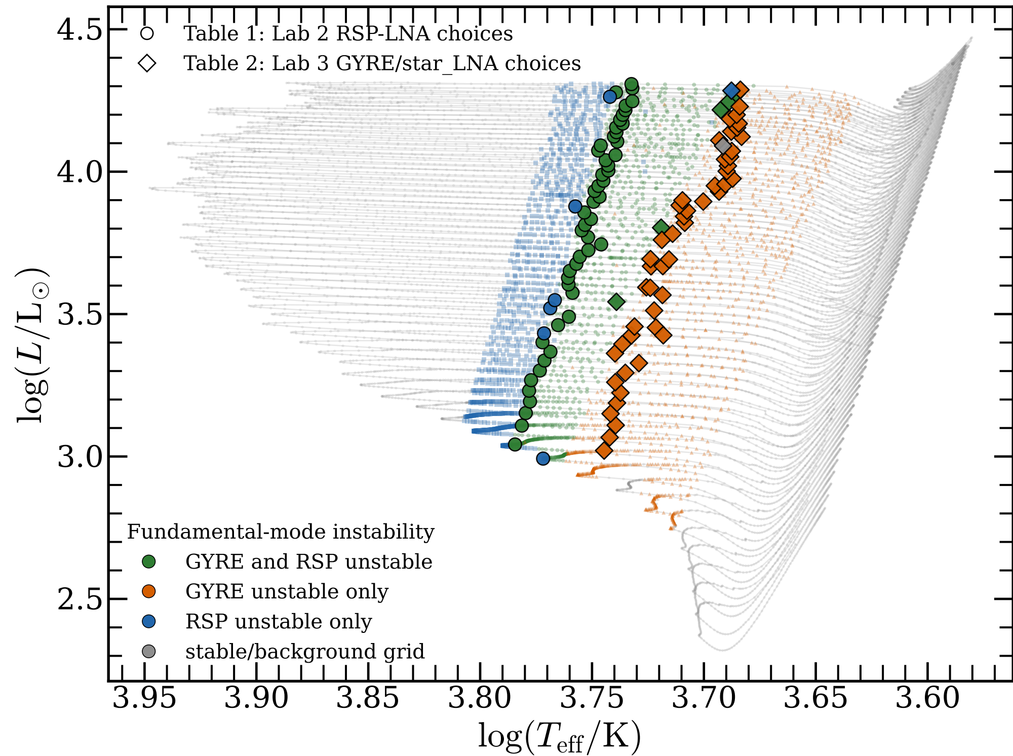
Lab 2 and Lab 3 model choices on the HR diagram
