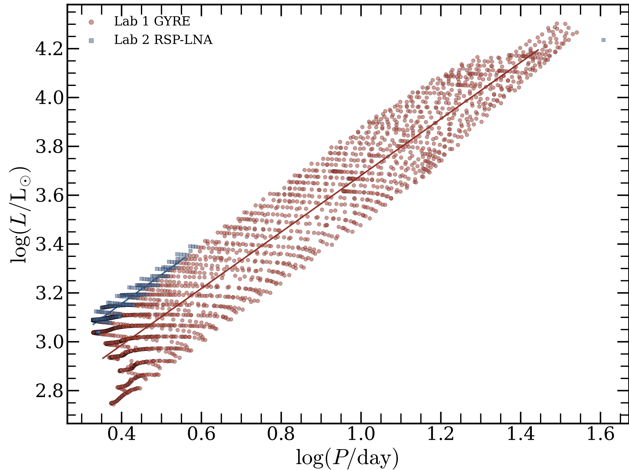
F_1 unstable, F_2 subdominant period-luminosity relation
