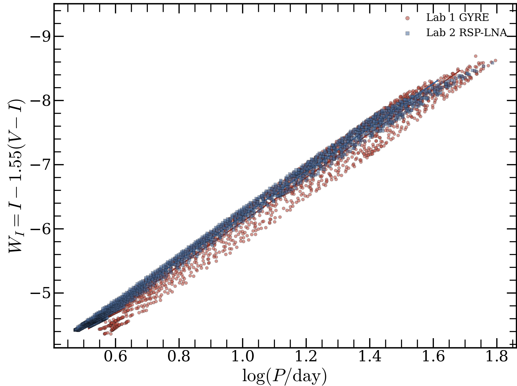
F_0 unstable, F_2 subdominant period-Wesenheit relation
