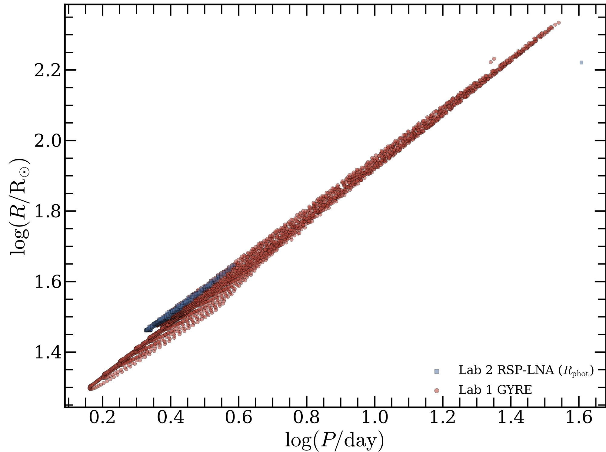
F_1 first-overtone unstable period-radius relation
